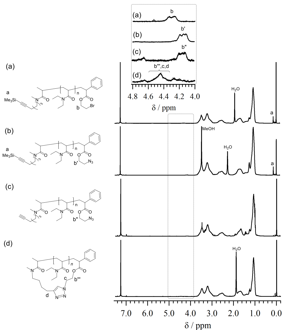
Figure 3-8. ^1\text{H} NMR spectra of (a) \text{Si}\equiv\text{-PDEAAm}_{50}\text{-Br} , (b) \text{Si}\equiv\text{-PDEAAm}_{50}\text{-N}_3 , (c) \equiv\text{-PDEAAm}_{50}\text{-N}_3 , and (d) \text{c-PDEAAm}_{50} in \text{CDCl}_3 (400 MHz).
