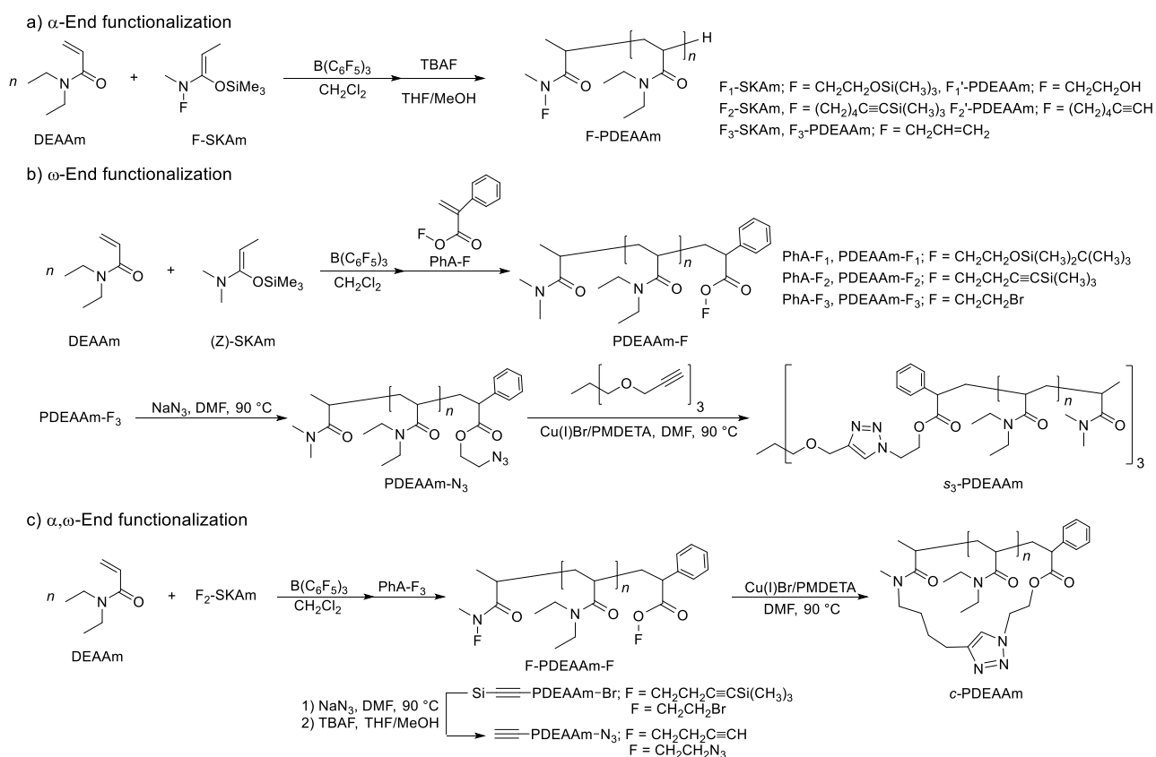
Scheme 3-1. Synthesis of Well-defined Linear, Cyclic, and Star-shaped PDEAAs Using \alpha -, \omega -, and \alpha,\omega -End-functionalized Poly( N,N -diethylacrylamide)s by B(C_6F_5)_3 -catalyzed Group Transfer Polymerization
