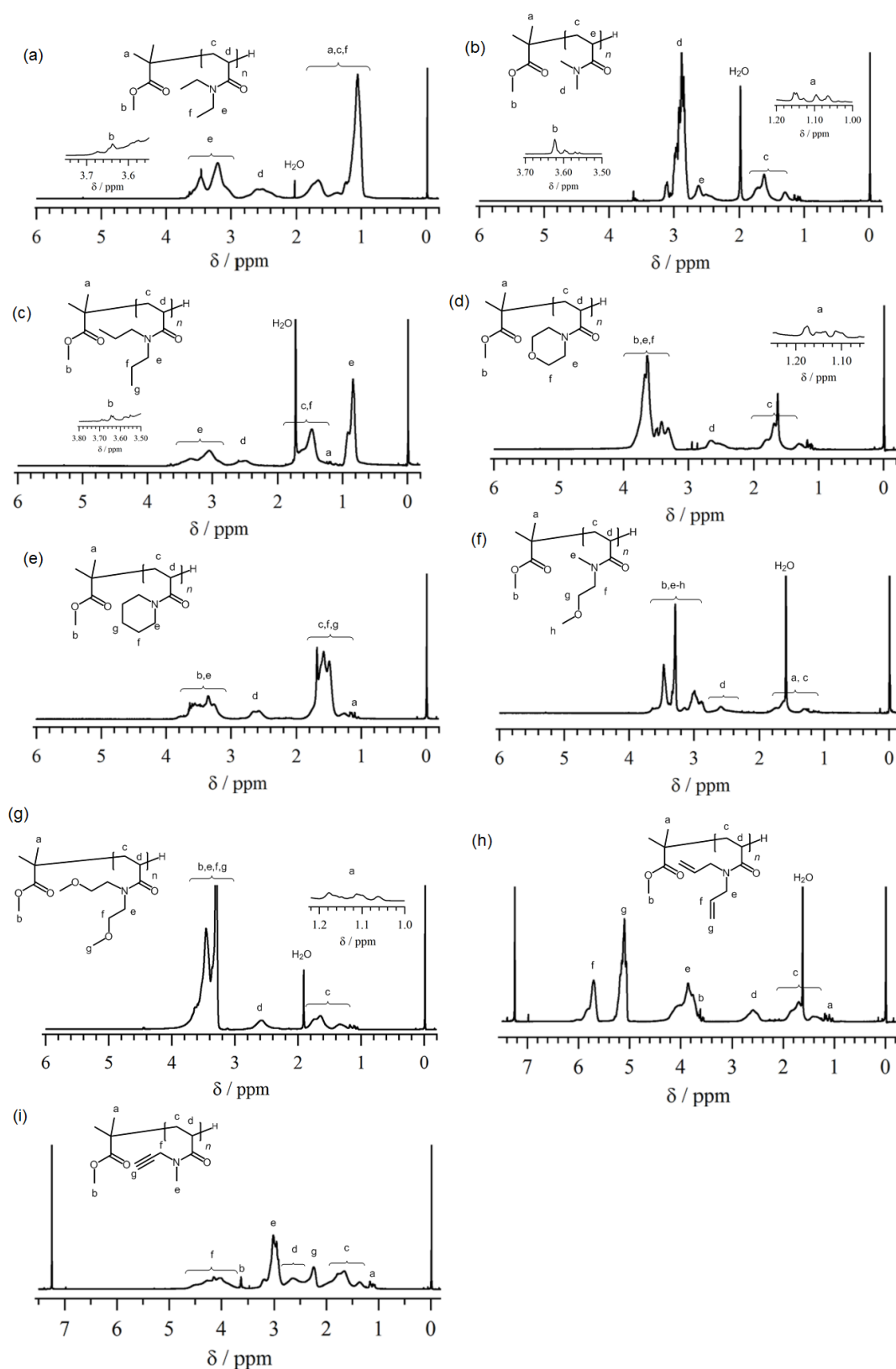
Figure 2-6. ^1\text{H} NMR spectra of (a) PDEAAm, (b) PDMAAm, (c) PDnPAAm, (d) PAPI, (e) PNAM, (f) PMMEAAm, (g) PBMEAAm, (h) PDALAAm, and (i) PMPAAm in \text{CDCl}_3 . (Theoretical DP, 25)
