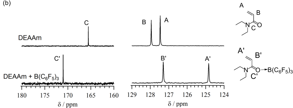
Figure 2-4. (a) ^1\text{H} and (b) ^{13}\text{C} NMR spectra of DEAAm and an equimolar mixture of DEAAm and \text{B}(\text{C}_6\text{F}_5)_3 ( [\text{DEAAm}]_0 = [\text{B}(\text{C}_6\text{F}_5)_3]_0 = 0.167 \text{ mol L}^{-1} ) in \text{CDCl}_3 .
