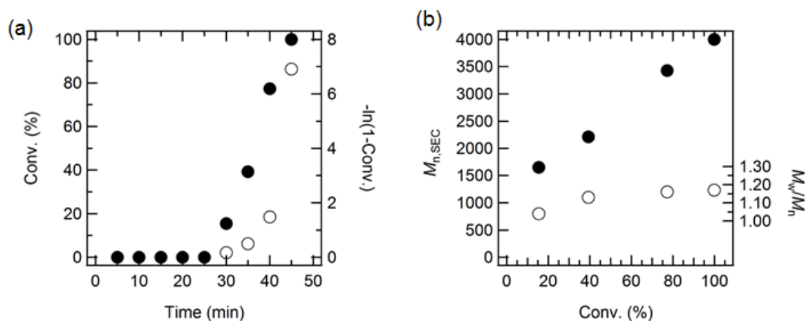
Figure 2-1. (a) Zero- (●) and first- (○) order kinetic plots of the \text{B}(\text{C}_6\text{F}_5)_3 -catalyzed GTP of DEAAm at 25 °C under the conditions of [\text{DEAAm}]_0/[\text{SKA}^{\text{Et}}]_0/[\text{B}(\text{C}_6\text{F}_5)_3]_0 = 25/1/0.05 and [\text{DEAAm}]_0 = 0.50 \text{ mol L}^{-1} and (b) Dependence of M_{n,SEC} (●) and M_w/M_n (○) of the obtained PDEAAm on Conv..
