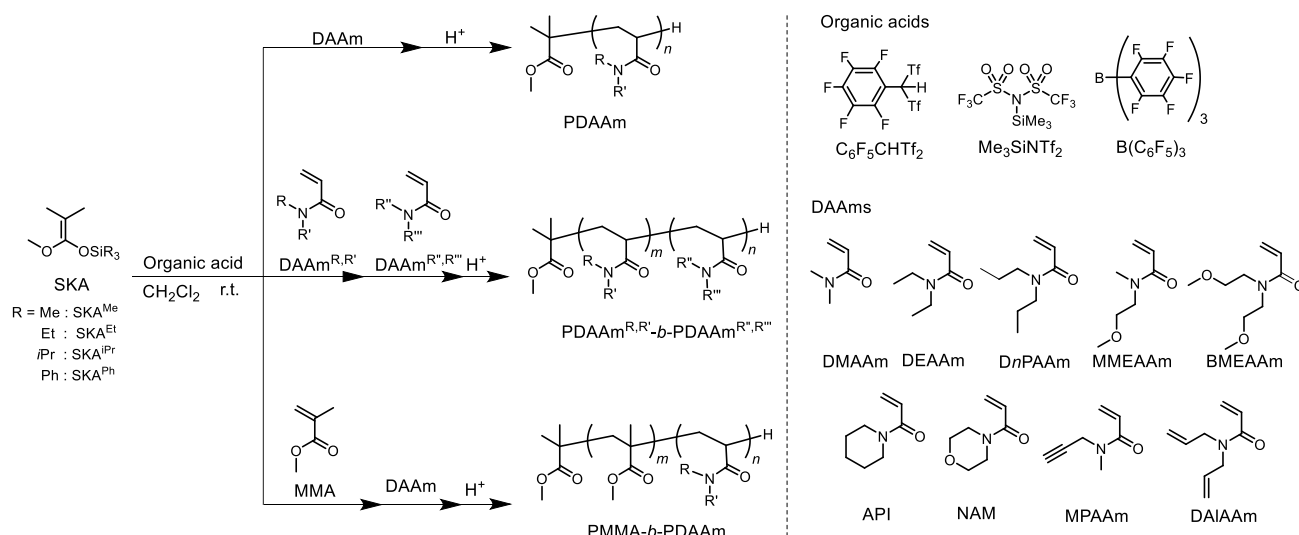
Scheme 2-1. Syntheses of homo acrylamide polymers, homo acrylamide block copolymers, and hetero block copolymers by organic acid-catalyzed group transfer polymerization method.
