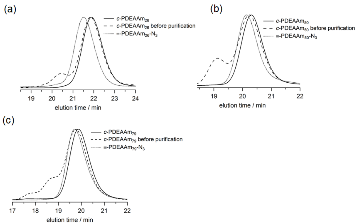
Figure 3-10. SEC traces of \equiv -PDEAAm- N_3 , its click reaction product, and c -PDEAAm (eluent, DMF containing 0.01 \text{ mol L}^{-1} \text{ LiCl} ; flow rate, 0.6 \text{ mL min}^{-1} ).
