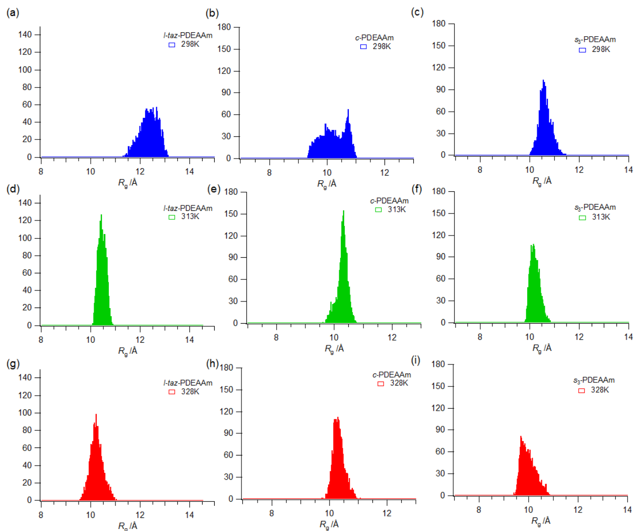
Figure 3-19. Histograms of R_g for l -taz-PDEAAm, c -PDEAAm, and s_3 -PDEAAm at 298 K (blue), 313 K (green), and 328 K (red) (last 5 ns data were used for the histogram).
