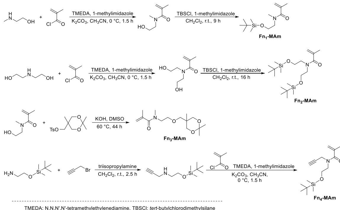
Scheme 4-2. Synthetic route of functional methacrylamides (Fn-MAMs).
