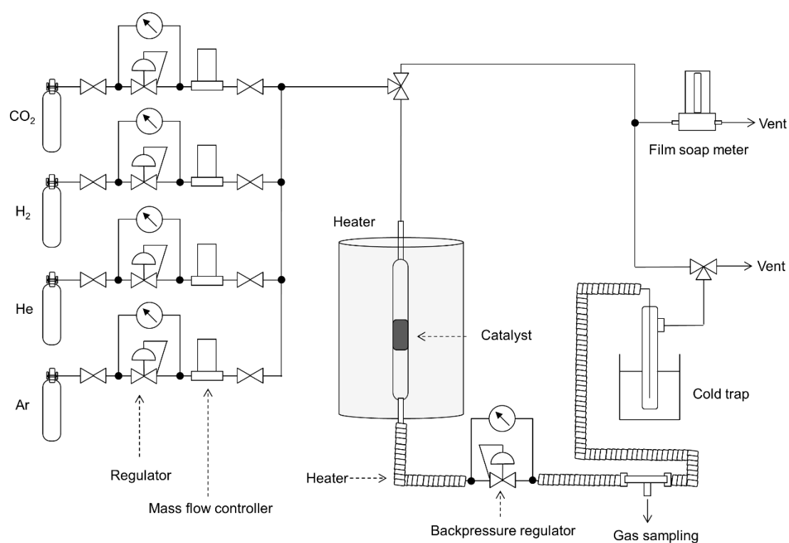
Figure 4.1. Fixed bed-flow reactor for hydrogenation of \text{CO}_2 .
