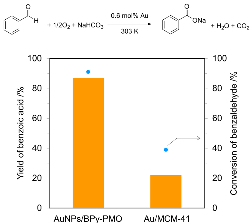
Figure 3.7. Aerobic oxidation of benzaldehyde in water with supported Au catalysts.
