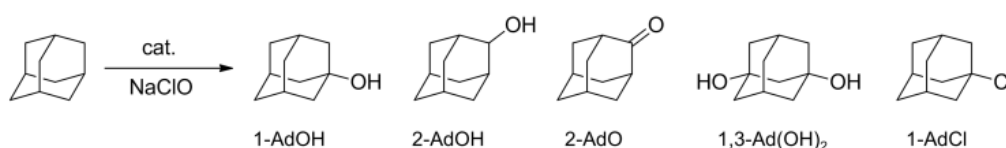
Scheme 2.3. Oxidation of adamantane with NaClO.
