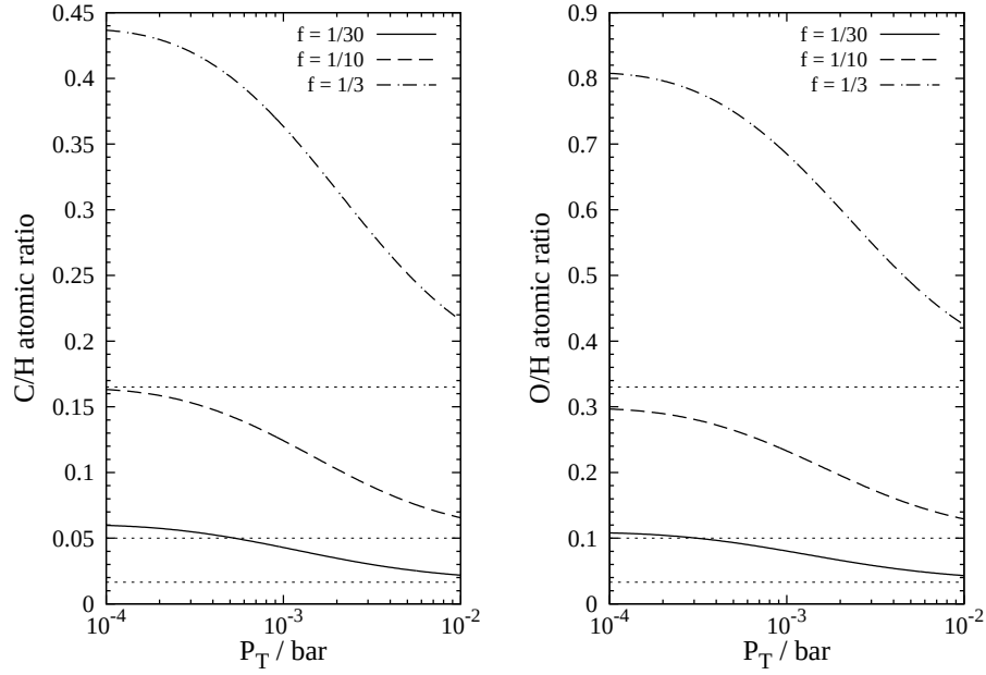
FIGURE 20 Elemental ratios, (C/H)_{\text{cell}} , (O/H)_{\text{cell}} , of carbon ( left ) and oxygen ( right ) relative to hydrogen in the sample room for f = 1/30 (solid line), 1/10 (dashed line), and 1/3 (dashed-dot line) at 1400^\circ\text{C} , as a function of P_T . Dotted lines represent the inlet (= outlet) ratios, (C/H)_0 , (O/H)_0 , for respective f values.
