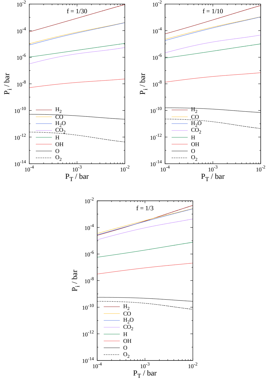
FIGURE 18 Partial pressures P_i of species i inside the sample room for f = 1/30 (top left), 1/10 (top right), and 1/3 (bottom) at 1400^\circ\text{C} , as a function of P_T .
