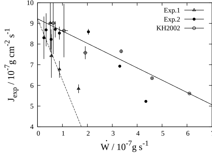
FIGURE 15 Results in the hydrogen experiment for P_{H_2} = 1.88 \cdot 10^{-4} atm at 1400^\circ\text{C} , compared with those of KH2002 and the regression curve (solid line) in the same condition. Also shown is a predicted evaporation rate (dashed line) for the present study, estimated from KH2002 using a change in the conductance of outlet tubes.
