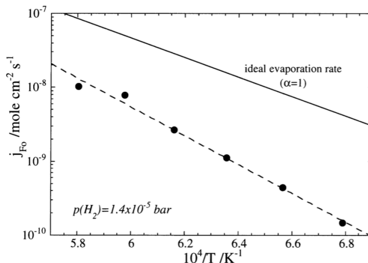
FIGURE 3 Arrhenius plot of the evaporation rate j_{\text{Fo}} for P_{\text{H}_2} = 1.4 \cdot 10^{-5} bar, obtained by Tsuchiyama et al. (1998). Also shown are ideal evaporation rates ( \alpha = 1 ) derived from the equilibrium vapor pressure at that temperature.
