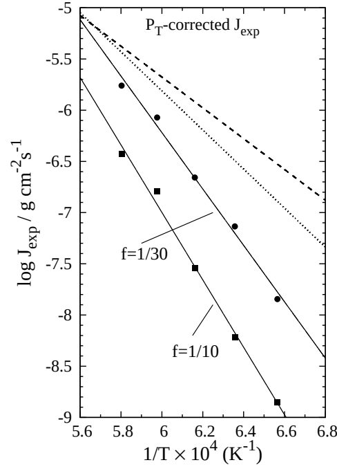
FIGURE 25 Arrhenius plots of J_{\text{exp}} of Fo for f = 1/30 (circle) and 1/10 (square) corrected for a constant P_T of 8.9 \cdot 10^{-4} bar. Dashed and dotted lines are the regression curves of J_{\text{exp}} for the present study and J_F for Kuroda and Hashimoto (2002) in a pure hydrogen for the same P_T condition, respectively.
