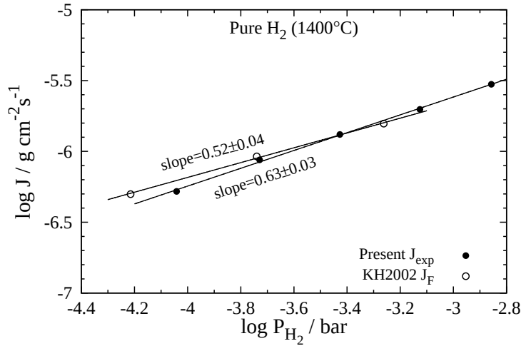
FIGURE 16 Evaporation rates J_{\text{exp}} in the present study and forward reaction rates J_F between Fo and atomic H in KH2002 at 1400°C, shown as a function of P_{\text{H}_2} .
