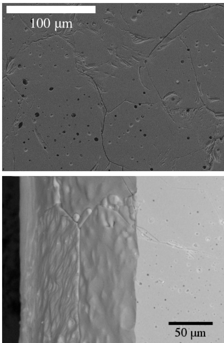
FIGURE 9 Back-scattered electron (BSE) images of starting samples, ( top ) showing a surface region of polycrystalline Fo minerals with grain boundaries and some pits on the surface, and ( bottom ) showing the cross section of the inside and the surface structure without polishing, which are separated each other by a boundary vertical line in the center of the figure. The surface topography is briefly inspected in this figure to verify that the region is free from rough structures on the surface with its less uphill and downhill.
