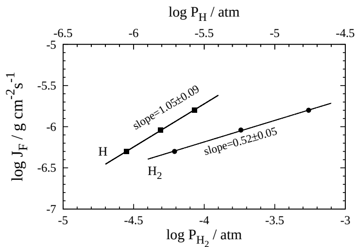
FIGURE 6 Reaction rates J_F of solid Fo with atomic H in hydrogen atmosphere at 1400°C, shown as functions of P_{\text{H}_2} (lower abscissa) and P_{\text{H}} (upper abscissa) in respective pressure scales. Dissociation equilibrium is assumed between \text{H}_2 and H.
