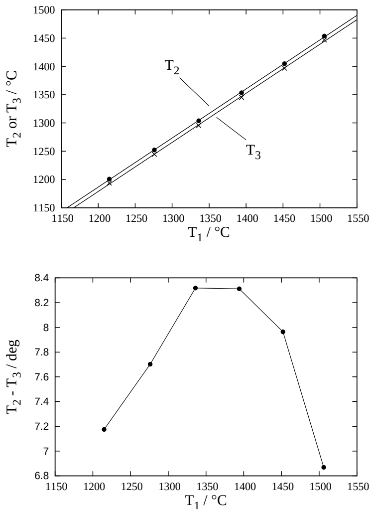
FIGURE 12 Temperatures measured without a sample and gas in the reaction room. T_1 is the temperature measured by the Type B thermocouple on the outer wall of the alumina tube near the reaction cell. T_2 is measured by the Type B thermocouple on the outer wall of the reaction cell near the site where a sample is set. T_3 is measured by the Type R thermocouple at the sample site. Measurement errors of these thermocouples are within \pm 0.5 deg.
