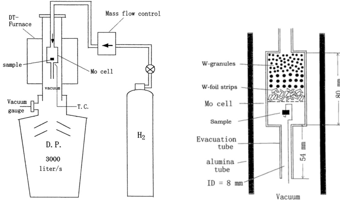
FIGURE 4 Left ): Experimental system for the solid-hydrogen reaction used by Kuroda and Hashimoto (2002). T.C.: thermocouple. D.P.: diffusion pump. DT-Furnace: Deltech DT-31-VT-68-C furnace. Right ): Inside view of the reaction cell.
