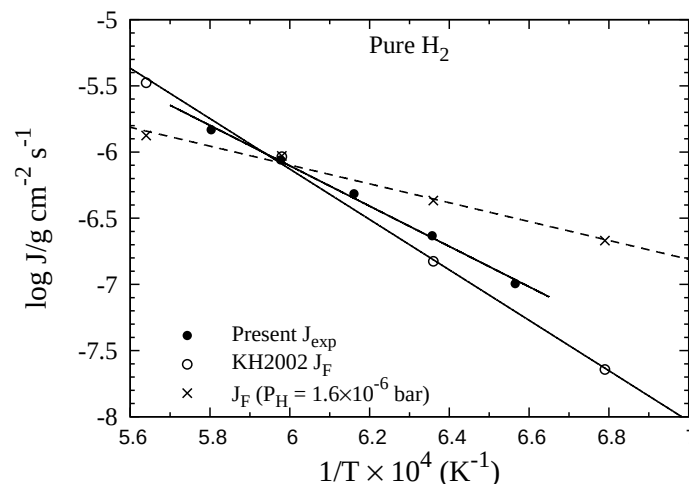
FIGURE 17 Comparison of the present study ( J_{\text{exp}} ) and KH2002 ( J_F ) for the evaporation rate of forsterite in pure hydrogen atmosphere.
