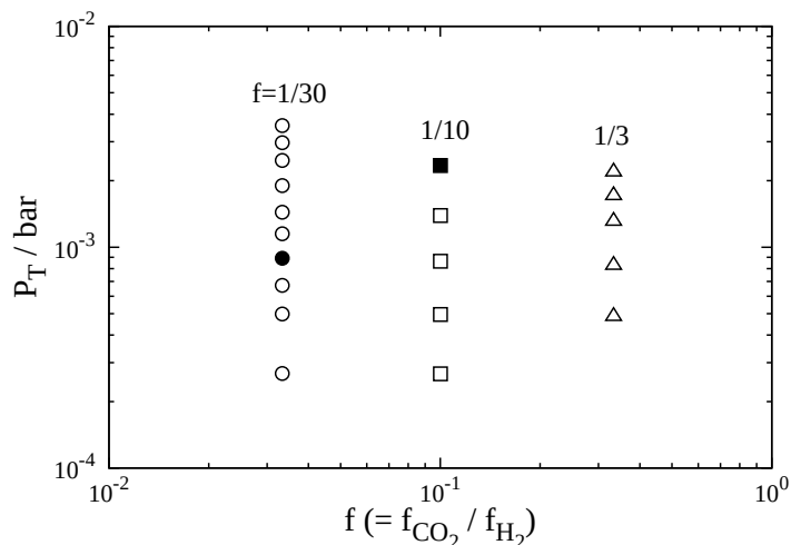
FIGURE 14 Experimental conditions in the mixing gas experiment. This P_T variation is achieved modifying the H_2 and CO_2 gas flow rates at 1400^\circ C . Filled symbols represent the nearly same conditions in varied temperature experiments ( 1250, 1300, 1350, 1400, 1450^\circ C ).
