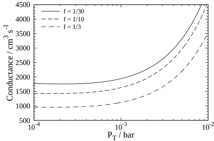
FIGURE 21 Mean conductance of the outlet tube (ID = 3.86 mm; L = 30.38 mm) for f = 1/30 (solid line), 1/10 (dashed line), and 1/3 (dot-dashed line) at 1400^\circ\text{C} ; weighted means in accordance with abundances of coexisting molecular species.
