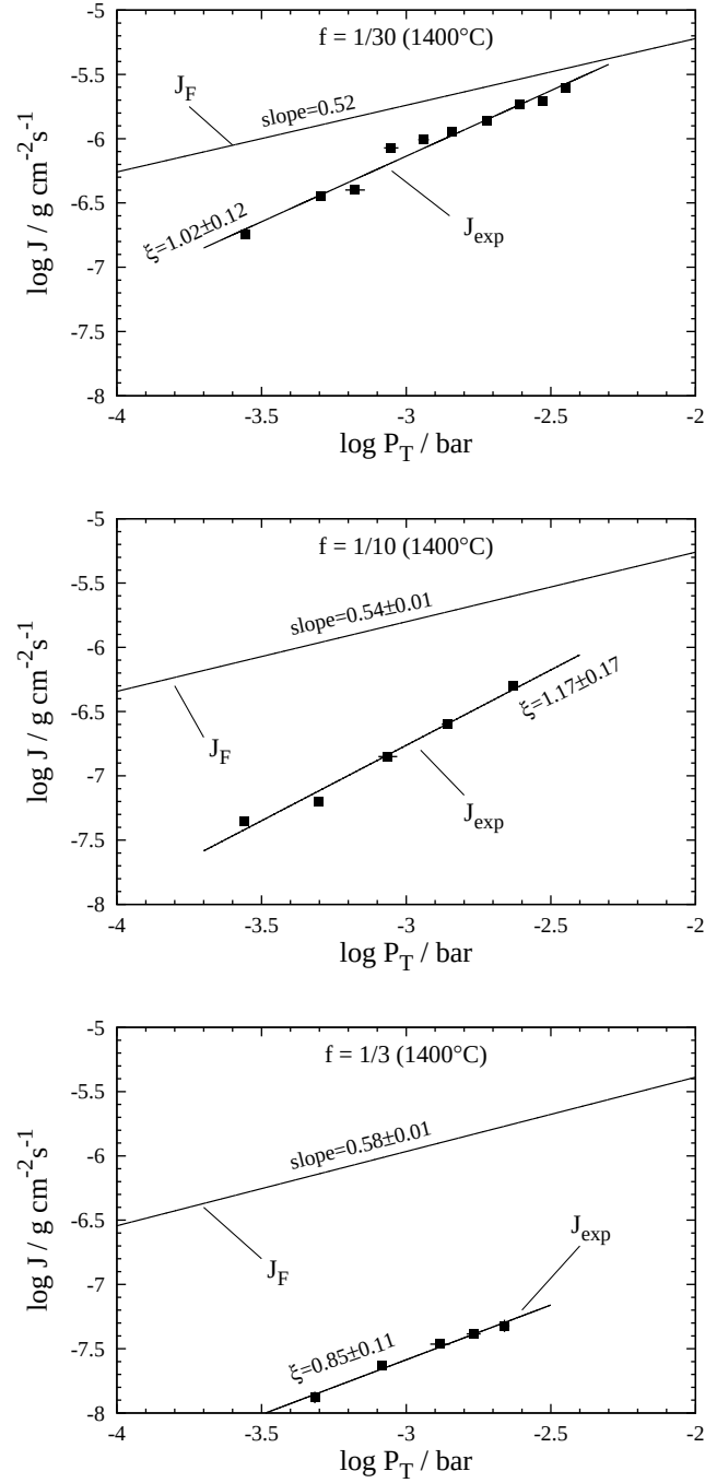
FIGURE 26 Comparison of J_{exp} and J_F for f = 1/30 (top), 1/10 (middle), and 1/3 (bottom) at 1400^\circ\text{C} .
