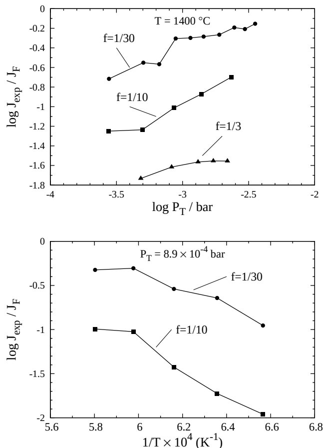
FIGURE 27 The systematic variation of J_{\text{exp}} in f relative to reaction rates J_F between Fo and atomic H, as functions of P_T at 1400^\circ\text{C} (top), and 1/T for P_T = 8.9 \cdot 10^{-4} \text{ bar} (bottom).
