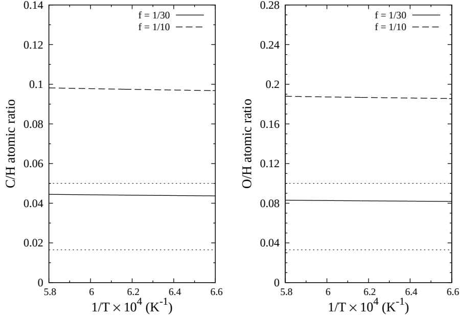
FIGURE 22 Elemental ratios, (C/H)_{\text{cell}} , (O/H)_{\text{cell}} , of carbon ( left ) and oxygen ( right ) relative to hydrogen in the sample room for f = 1/30 with f_{\text{H}_2} = 17.0 and f_{\text{CO}_2} = 0.57 cc/min at STP (solid line), and for f = 1/10 with f_{\text{H}_2} = 45.7 and f_{\text{CO}_2} = 4.57 cc/min at STP (dashed line), as a function of 1/T . Dotted lines represent the inlet (= outlet) ratios, (C/H)_0 , (O/H)_0 , for respective f values.
