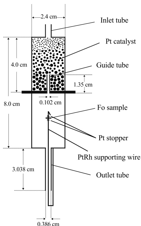
FIGURE 11 Schematic illustration of the reaction cell.
