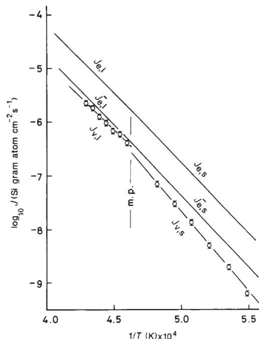
FIGURE 1 Evaporation rates J_{v,s} and J_{v,l} (open circles) of forsterite (Fo) in vacuum, measured by Hashimoto (1990) for temperatures T above and below the melting point (m.p.), respectively. J_{v,s} is the evaporation rate of solid Fo and J_{v,l} is that for liquid Fo (denoted by the subscript s for solid and the subscript l for liquid). The ideal evaporation rate J_e for \alpha_v = 1 calculated using the equilibrium Fo vapor pressures is shown for comparison.
