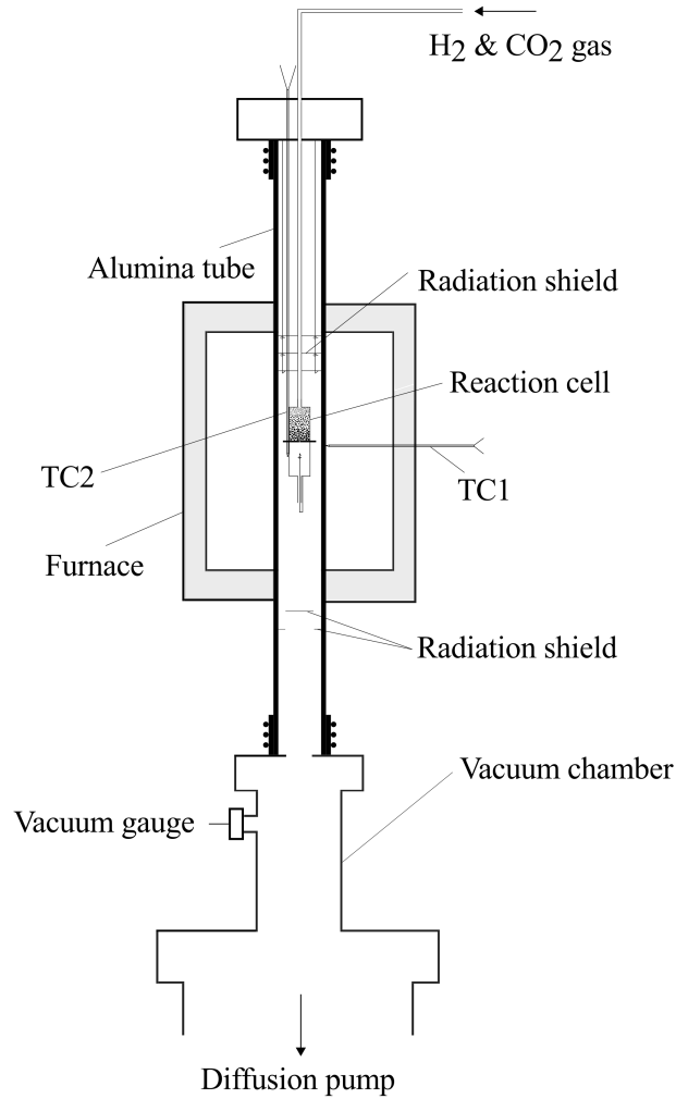
FIGURE 10 Experimental assembly.
