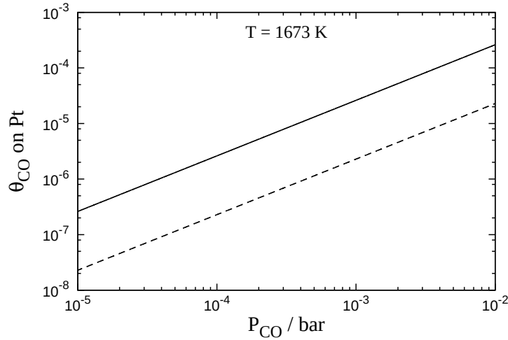
FIGURE 32 Coverage \theta_{\text{CO}} of CO adsorbate as a function of P_{\text{CO}} at 1673 K. Solid and dashed lines represent the best estimate of \theta_{\text{CO}} expected for pre-exponential factor \nu_{\perp, \text{CO}} = 1.25 \cdot 10^{15} \text{ s}^{-1} , and desorption energies E_{\text{d,CO}} = 43 and 34.9 \text{ kcal/mol} , respectively. Total number N_{\text{site}} of site on Pt is assumed to be 1.54 \cdot 10^{15} \text{ cm}^{-2} .
