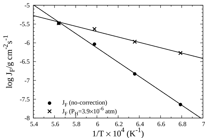
FIGURE 7 Arrhenius plot of the true evaporation rate J_F as a function of the inverse temperature 1/T in a hydrogen flow rate of 20 cc/min at the standard state (1 atm, 20°C). Filled circles and crosses show the values of J_F without and with the pressure correction, respectively. See text for the details.
