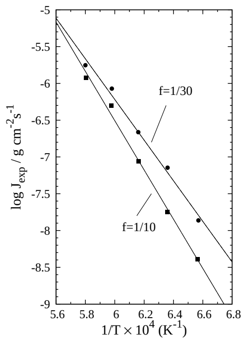
FIGURE 24 Arrhenius plots of J_{\text{exp}} for f = 1/30 ( f_{\text{H}_2} = 17.0 and f_{\text{CO}_2} = 0.56 cc/min at STP), and for f = 1/10 ( f_{\text{H}_2} = 45.7 and f_{\text{CO}_2} = 4.57 cc/min at STP).
