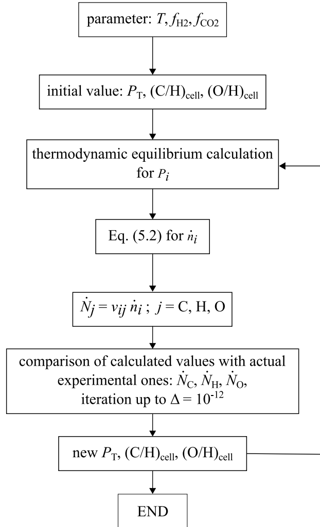
FIGURE 13 Flow chart of the numerical calculation for the derivation of gaseous pressure in the sample room. \Delta is the iteration accuracy, for which we took \Delta = 10^{-12} .
