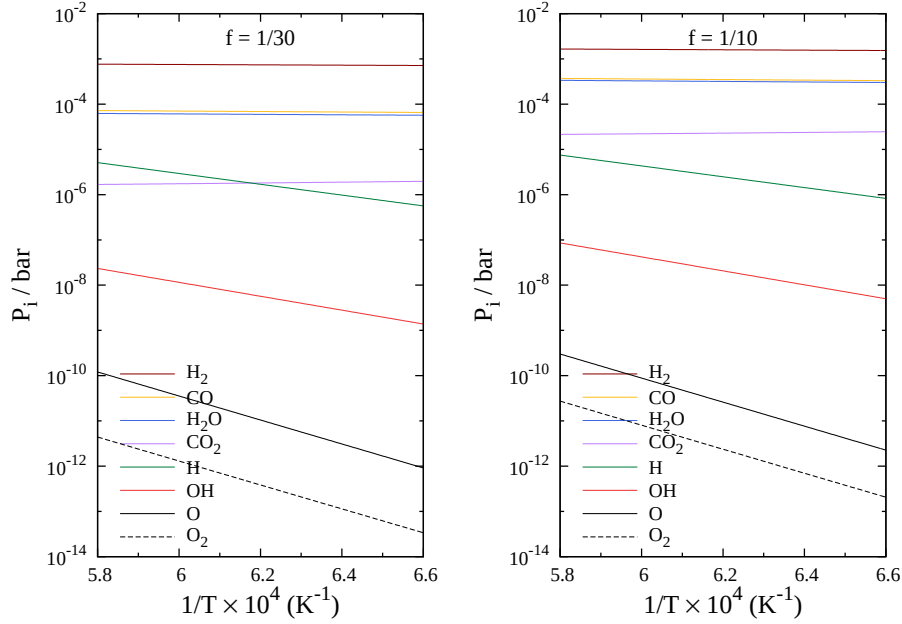
FIGURE 19 Partial pressures P_i of species i for f = 1/30 with f_{\text{H}_2} = 17.0 and f_{\text{CO}_2} = 0.56 cc/min at STP (left), and for f = 1/10 with f_{\text{H}_2} = 45.7 and f_{\text{CO}_2} = 4.57 cc/min at STP (right), as a function of 1/T .
