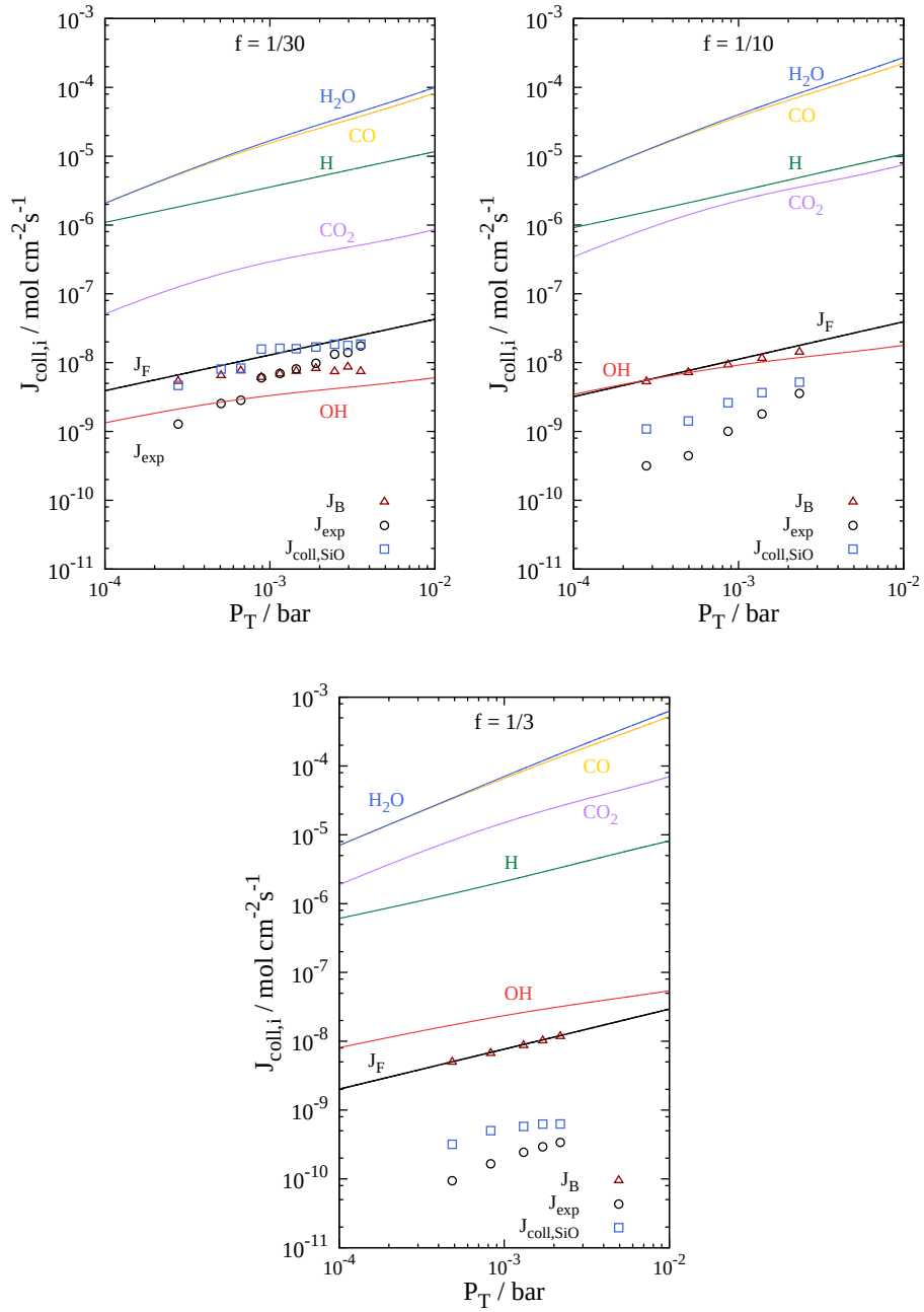
FIGURE 29 Collision rates J_{\text{coll},i} of the relevant species i for f = 1/30 (top left), 1/10 (top right), and 1/3 (bottom) at 1400^\circ\text{C} , compared with the condensation flux J_B when J_1 = J_F is assumed. Also shown are the data for J_{\text{exp}} and J_F .
