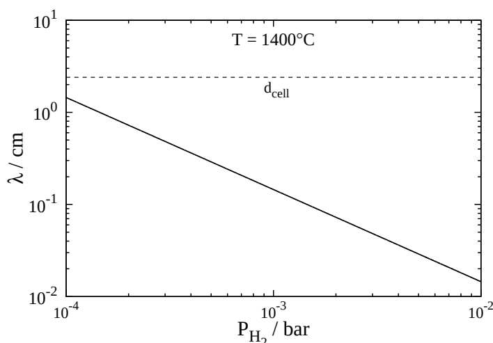
FIGURE 33 Mean free path \lambda of SiO in terms of H_2 collision at 1400°C.
