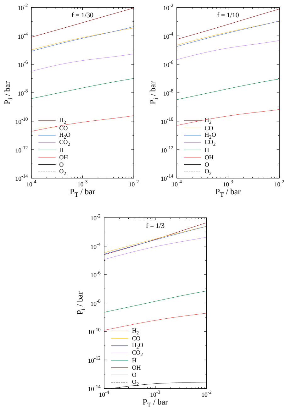
FIGURE 30 Partial pressures P_i of species i for f = 1/30 (top left), 1/10 (top right), and 1/3 (bottom) at 1400^\circ\text{C} with the equilibrium composition of molecules in the upper catalytic room assumed.
