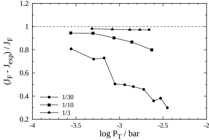
FIGURE 28 (J_F - J_{\text{exp}})/J_F for f = 1/30, 1/10 , and 1/3 at 1400^\circ\text{C} , as a function of P_T . If J_B = J_F - J_{\text{exp}} , a dashed line ( J_B/J_F = 1 ) represents a balance between evaporation and condensation.
