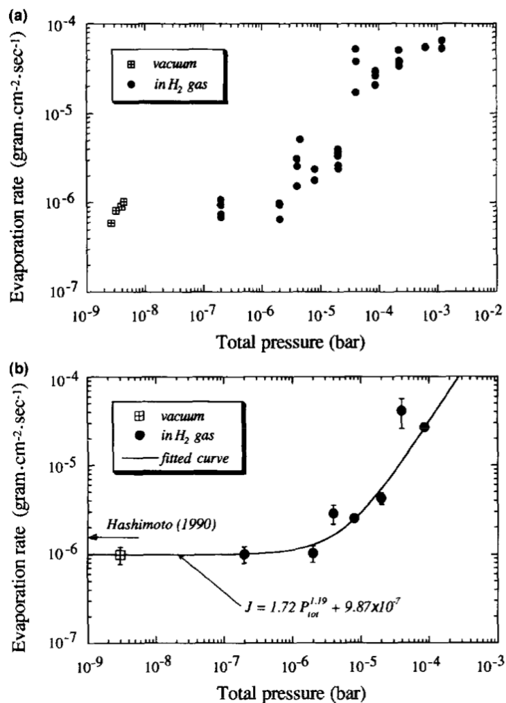
FIGURE 2 Evaporation rate J versus hydrogen pressure P_{\text{H}_2} (filled circle) and that in vacuum (open square) at 1700^\circ\text{C} , obtained by Nagahara and Ozawa (1996). Graph (a) represents the measured evaporation rates and (b) the optimized evaporation rates. The evaporation rate in vacuum by Hashimoto (1990) is shown by an arrow.
