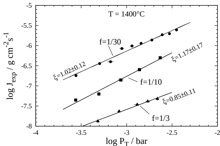
FIGURE 23 Evaporation rates J_{\text{exp}} for the mixing ratios f = 1/30 (circle), 1/10 (square), and 1/3 (triangle) at 1400^\circ\text{C} . Slopes \xi (= d \log J_{\text{exp}} / d \log P_T) of the regression curves are represented for each f value.
