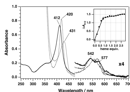
Fig. 1 Absorption spectra of the heme-HutZ complex. The protein concentration is 5 \mu\text{M} (per heme basis) in 50 mM Tris-Cl/150 mM NaCl, pH 8.0. Spectra shown are in the ferric (solid line), ferrous (dotted line), and CO-bound forms (dashed line). (Inset) Heme-binding curve generated from the difference absorbance spectra by plotting \Delta A_{412} vs. the molar ratios of hemin to the protein.
