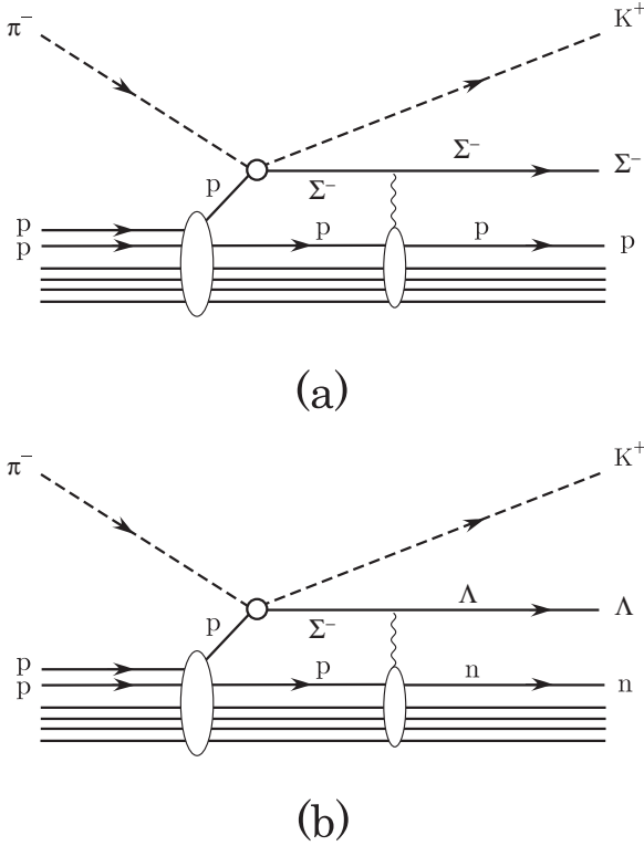
FIG. 1. Diagrams for double-charge exchange ( \pi^- , K^+ ) reactions on nuclear targets, leading to production of (a) \Sigma hypernuclear states by \pi^- p \rightarrow K^+ \Sigma^- processes and (b) \Lambda hypernuclear states caused by the \Sigma^- p \leftrightarrow \Lambda n coupling.
