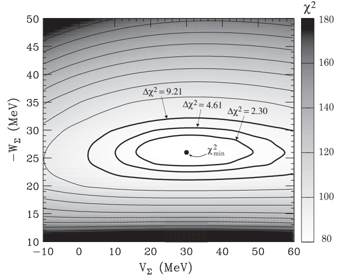
FIG. 6. Contour plots of the \chi^2 -value distribution in the \{V_\Sigma, -W_\Sigma\} plane from fitting to the average cross section of \bar{\sigma}_{2^\circ-14^\circ} in the {}^6\text{Li}(\pi^-, K^+) reaction at p_{\pi^-} = 1.2 GeV/ c . A solid circle denotes the minimum position of \chi_{\text{min}}^2 = 84.5 at (V_\Sigma, -W_\Sigma) = (30 \text{ MeV}, 26 \text{ MeV}) with f_s = 1.23 . Thick curves indicate \Delta\chi^2 = 2.30, 4.61 , and 9.21 which correspond to 68%, 90%, and 99% confidence levels for two parameters, respectively.
