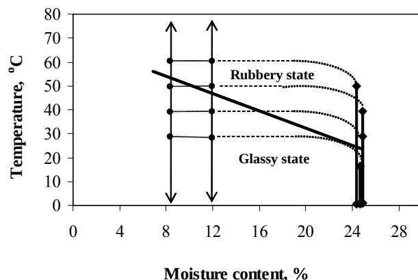
Fig. 3. Macroscopic indications of kernel states during the drying process
