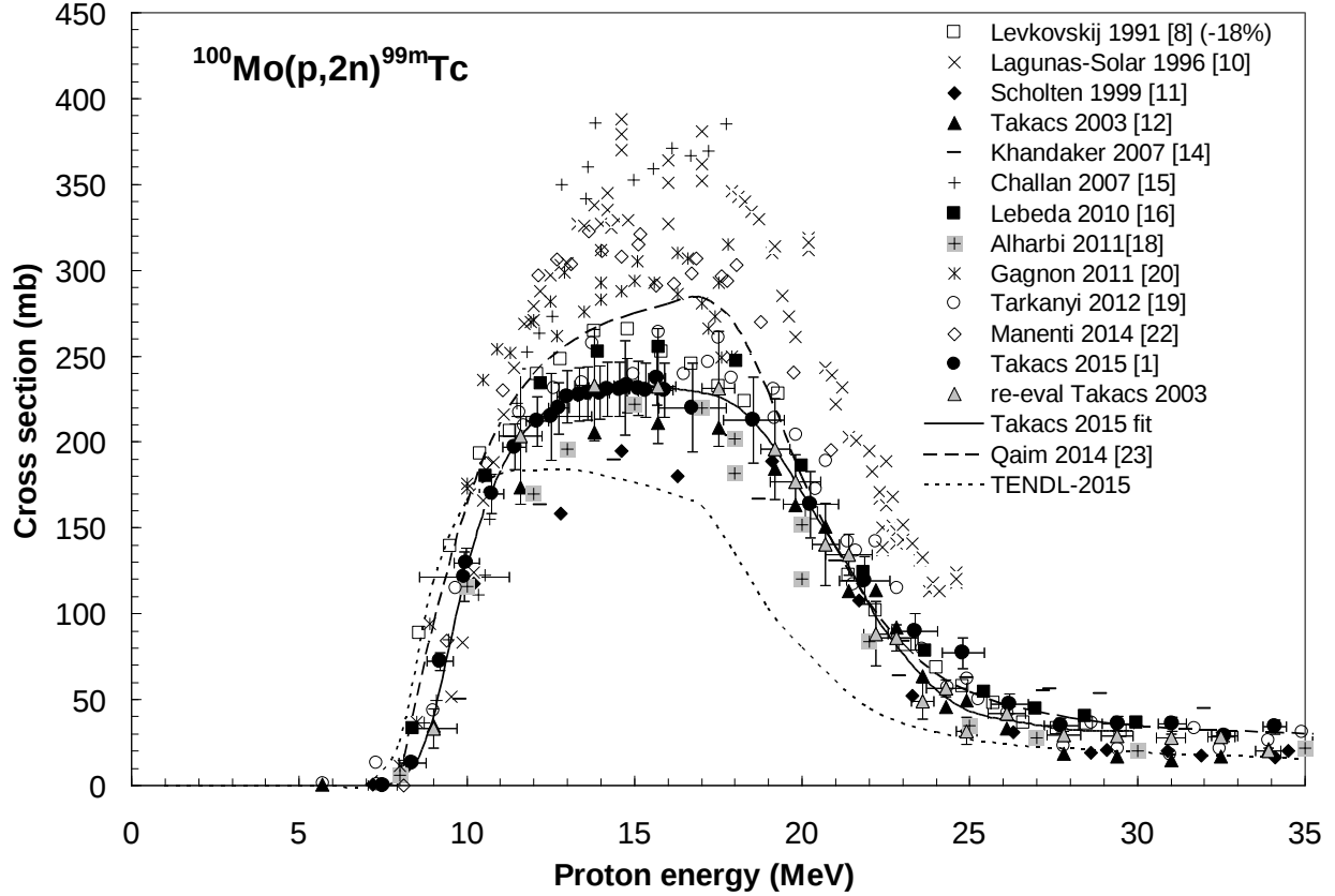
Figure 1. Available experimental and evaluated cross section data for the ^{100}\text{Mo}(p,2n)^{99\text{m}}\text{Tc} reaction.
