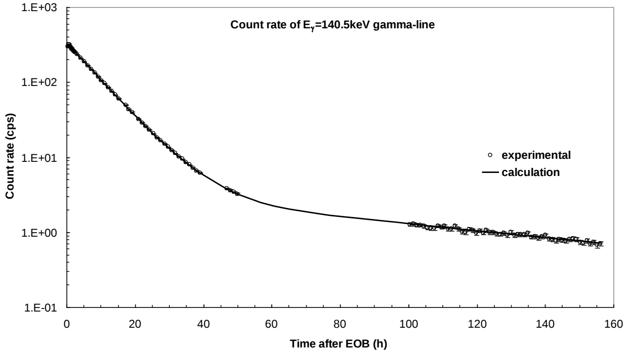
Figure 4. Count rate determined for the E_\gamma = 140.5 keV gamma-line in a thick Mo target irradiated with a 17.9 MeV proton beam. Open symbols: experimental values, solid line: calculated curve based on the cross sections published in [1].
