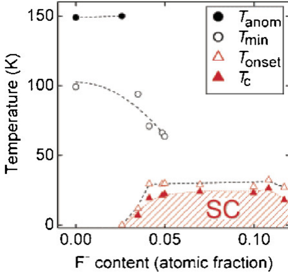
Figure 1.1: The phase diagram of \text{LaFeAsO}_{1-x}\text{F}_x [19].
