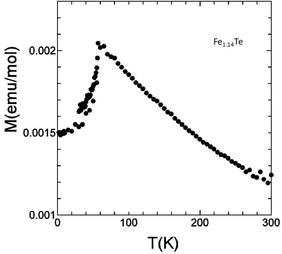
Figure 3.2: Temperature dependence of the magnetic susceptibility on \text{Fe}_{1.14}\text{Te} . There is large reduction of magnetic susceptibility around 58 K. Antiferromagnetic transition temperature is determined as 58 K.
