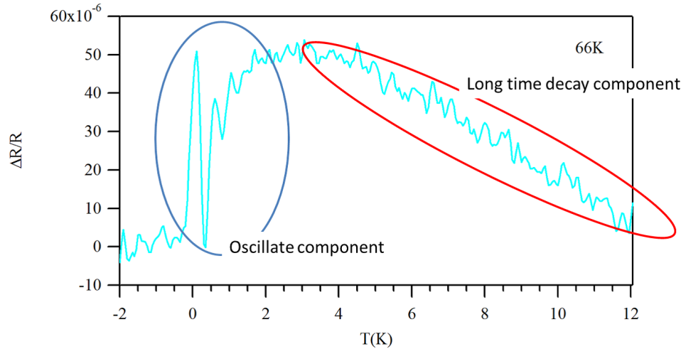
Figure 3.24: \Delta R/R at 66 K.
