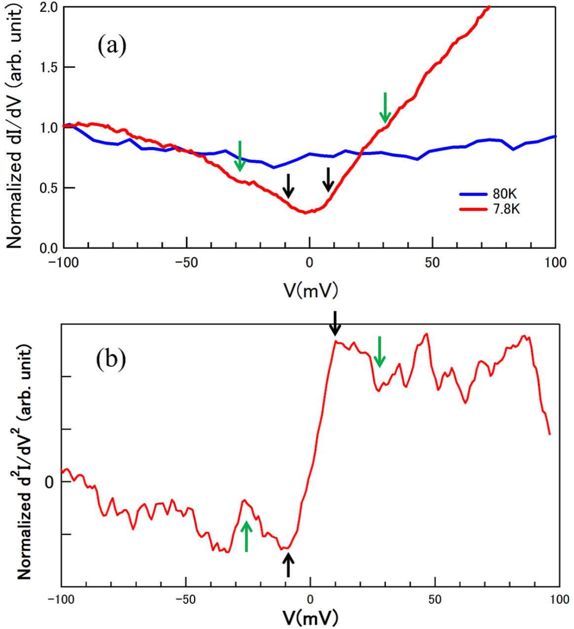
Figure 3.8: (a) Tunneling differential conductance on \text{Fe}_{1+x}\text{Te} ( x=0.14 ) at 7.8 K and 80 K indicated by red and blue line, respectively. Black and green arrows indicate the SDW gap and the pseudogap, respectively. (b) Numerical differential of the differential conductance on \text{Fe}_{1+x}\text{Te} ( x=0.14 ) at 7.8 K. Black arrows and green arrows correspond to the SDW gap and the pseudogap at the differential conductance curve. 2\Delta_{\text{SDW}}=18 meV.
