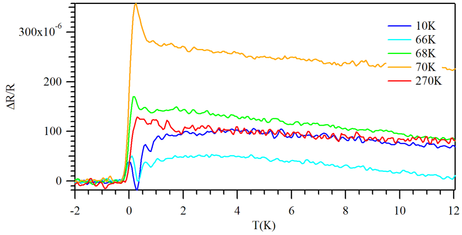
Figure 3.21: \Delta R/R transients at several temperatures from Fig.3.20.
