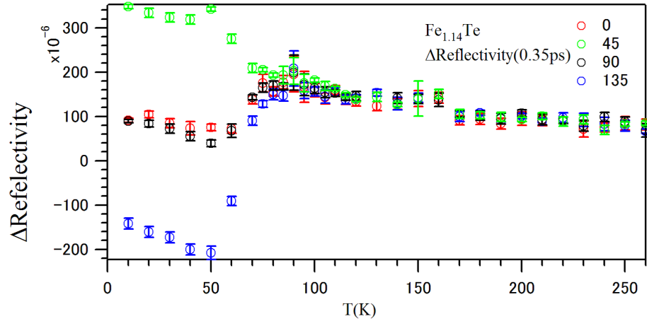
Figure 3.17: Temperature dependence of \Delta\text{Reflectivity} at 0.35 ps at 0, 45, 90 and 135 polarization.
