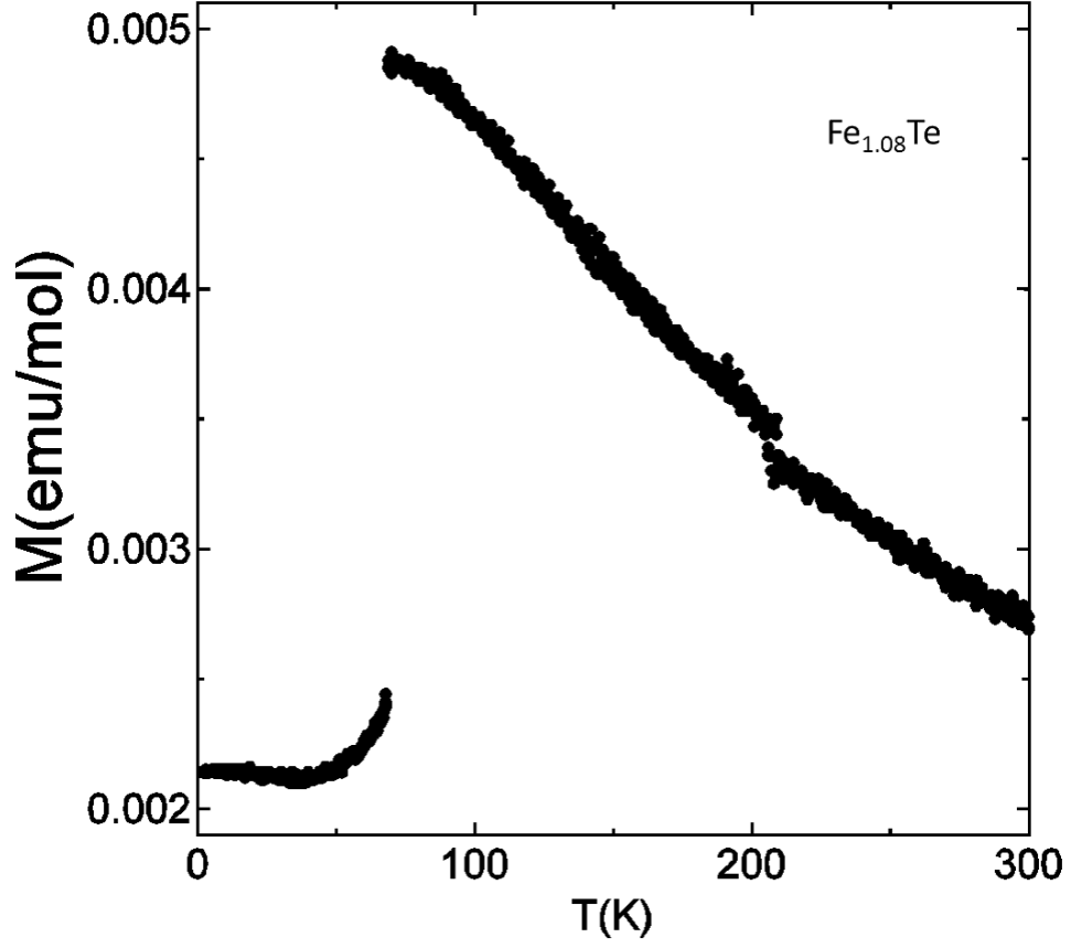
Figure 3.1: Temperature dependence of the magnetic susceptibility on \text{Fe}_{1.08}\text{Te} . There is large reduction of magnetic susceptibility around 68 K. Antiferromagnetic transition temperature is determined as 68 K.
