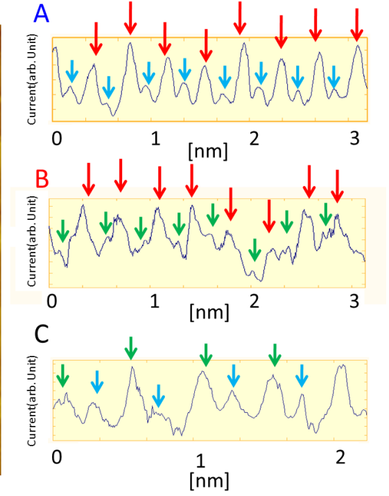
Figure 3.7: STM current image of \text{Fe}_{1+x}\text{Te} ( x=0.14 ) at bias voltage V = 700 mV and tunneling current I = 1.0 nA. The image is 3.3 nm square. There are line profiles in the STM image. A, B and C in the STM image correspond to the line profiles signs. Peaks indicated by green and blue arrows correspond to the tunneling current from Fe atoms. The red arrow peaks correspond to the tunneling current from Te atoms. The kinds of atoms are decided by atomic distance.
