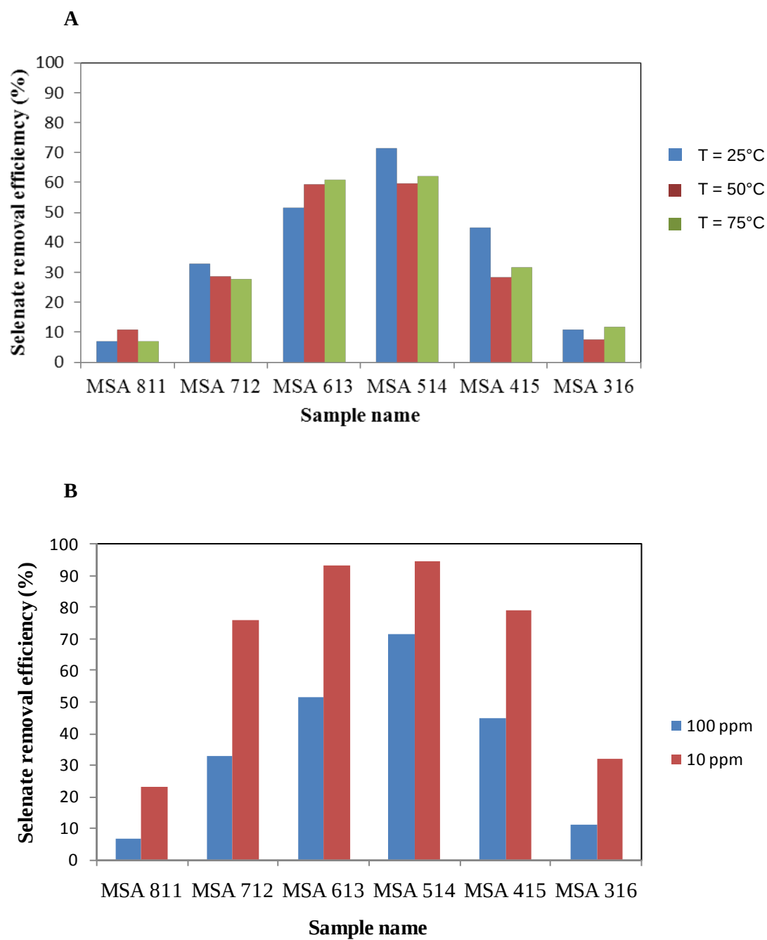
Figure 7 Comparison between the removal efficiency of co-precipitated selenate by the generated phases at different temperature conditions (A) and initial Se concentration (B).
