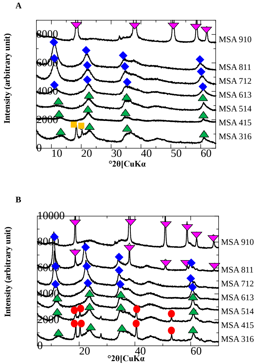
Figure 1 XRD patterns of pure synthesized Mg-bearing minerals at 25°C and 75°C. ▼ brucite ♦ hydrotalcite ▲ serpentine ● gibbsite ■ bayerite
