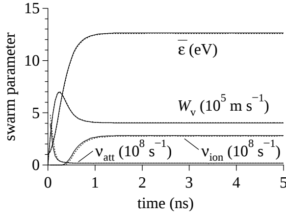
Figure 9. Physical relaxation process of mean electron energy \bar{\epsilon} , drift velocity W_v , ionization frequency \nu_{\text{ion}} and attachment frequency \nu_{\text{att}} in \text{SF}_6 at E/N = 1000 \text{ Td} ( E = 353.6 \text{ V/cm} , 133 \text{ Pa} at 273 \text{ K} ). Broken curves, MC; and solid curves, PM. The propagator operation was repeated 10^5 times for the simulation of 5 \text{ ns} with \Delta t = 0.05 \text{ ps} .
