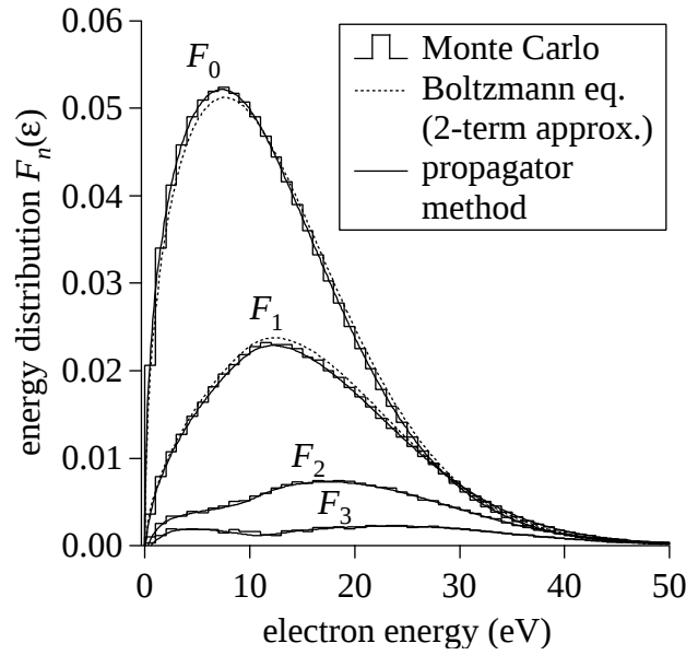
Figure 8. Electron energy distribution in \text{SF}_6 at E/N = 1000 \text{ Td} ( E = 353.6 \text{ V/cm} , 133 \text{ Pa} at 273 \text{ K} ): histograms, MC; broken curves, BE analysis (2-term approximation); and solid curves, PM. F_n(\epsilon) represents the n th order terms of Legendre polynomial expansion of the EEDF.
