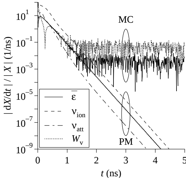
Figure 10. Decay of normalized time derivative |dX/dt|/|X| of a parameter X . X represents mean electron energy \bar{\epsilon} , drift velocity W_v , ionization frequency \nu_{\text{ion}} and attachment frequency \nu_{\text{att}} in \text{SF}_6 at E/N = 1000 \text{ Td} ( E = 353.6 \text{ V/cm} , 133 \text{ Pa} at 273 \text{ K} ). The MC results of \nu_{\text{ion}} and \nu_{\text{att}} are not shown because they fluctuated significantly.
