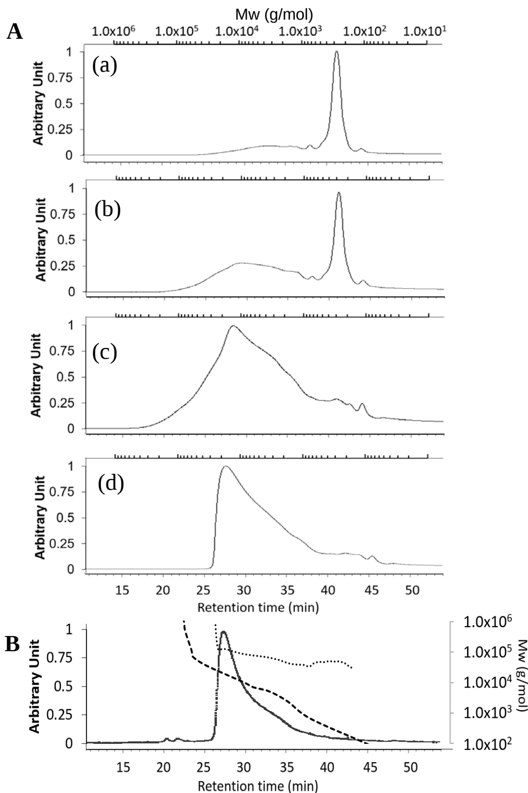
Fig. 3 Size exclusion chromatograms of EPEG-SL in chloroform. A series of chromatograms were monitored on a UV detector at 280 nm for the solution at the concentration of 0.5 mg/mL (a); 1.0 mg/mL (b); 2.0 mg/mL (c); and 3.0 mg/mL (d). Chromatogram B at the concentration of 3.0 mg/mL was monitored on a MALS detector. In B, calibration curves of absolute Mw and relative molecular mass were obtained by a direct measurement of specimen using the MALS detector and by using authentic polystyrene standards, respectively. A right Y-axis shows molecular mass for the calibration curves (—SEC chromatogram, .....calibration for absolute Mw, -----calibration for relative molecular mass)
