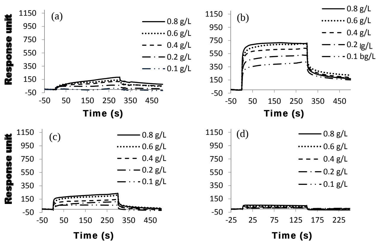
Fig. 6 Sensorgrams of EPEG-AL (a), EPEG-SL (b), EPEG-KL (c) and PEG 4000 (d) for CBH I immobilized on the sensor chip
