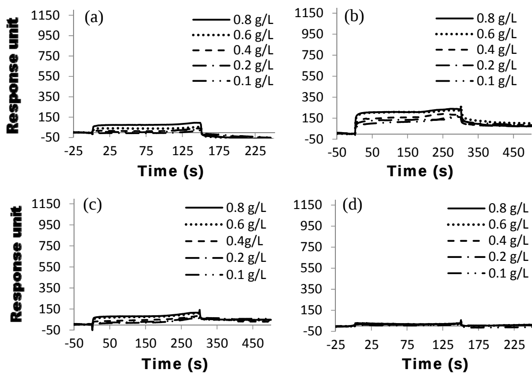
Fig. 8 Sensorgrams of EPEG-AL (a), EPEG-SL (b), EPEG-KL (c) and PEG 4000 (d) for EG I immobilized on the sensor chip
