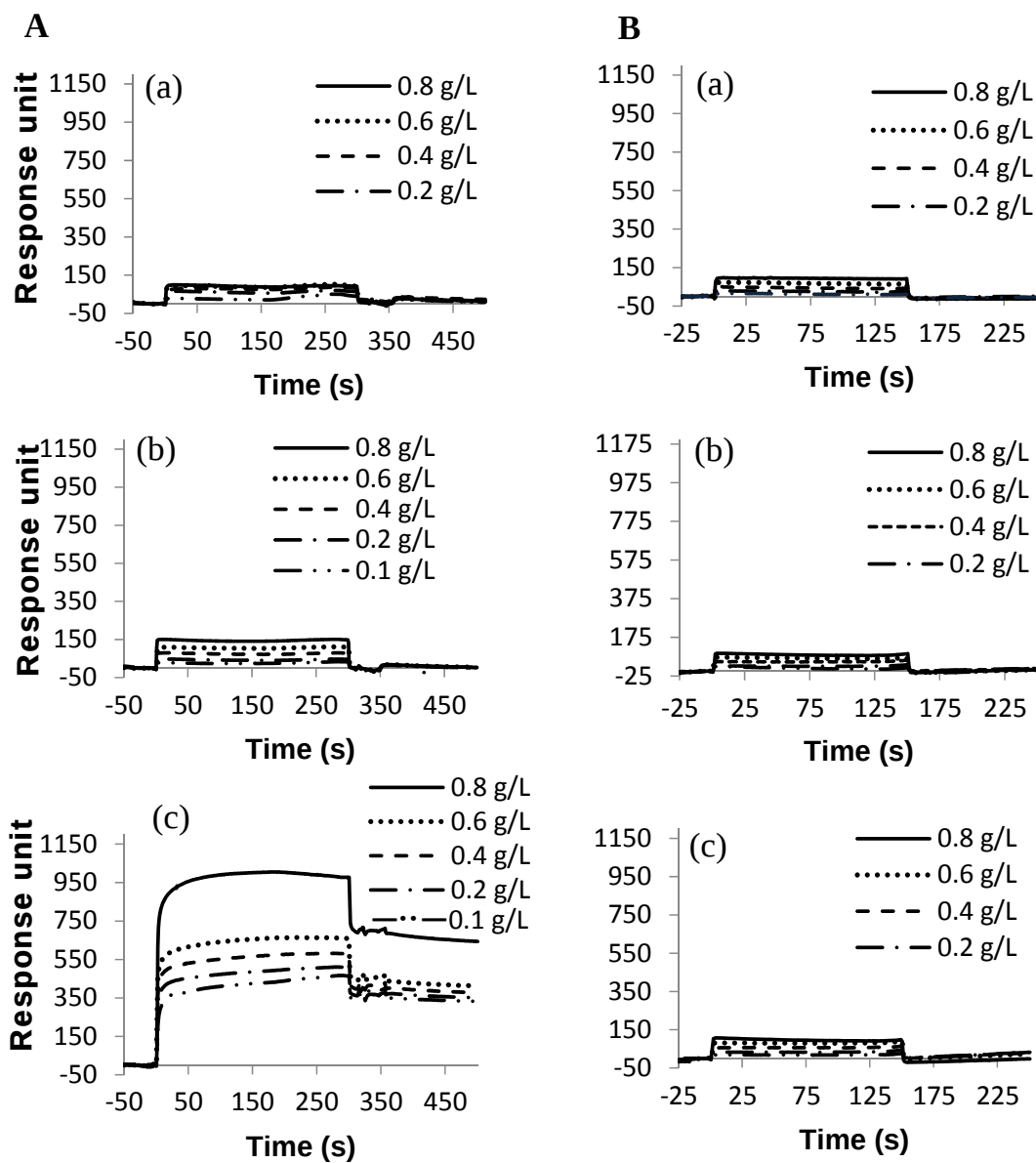
Fig. 5 Sensorgrams of EPEG-AL (A) and PEG 4000 (B) for various functional groups on sensor chips. (a), hydroxy group; (b), carboxy group; and (c), amino group
