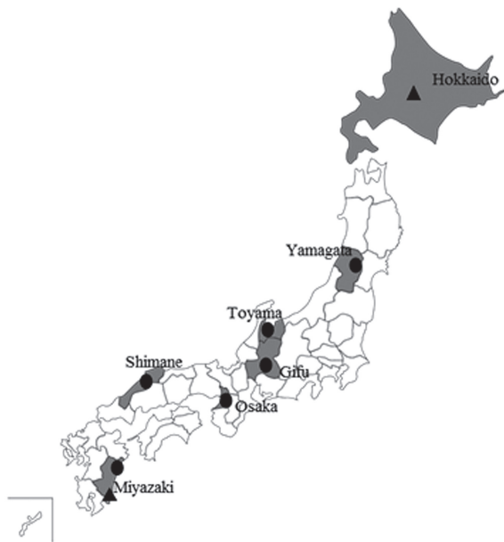
Fig. 1. Map showing the survey sites in Japan and animal species collected from each site. Rodents were collected from six prefectures (circles), while deer were collected from two sampling sites in northern and western Japan (triangles). The grey areas are the prefectures where sika deer and rodents were captured.
