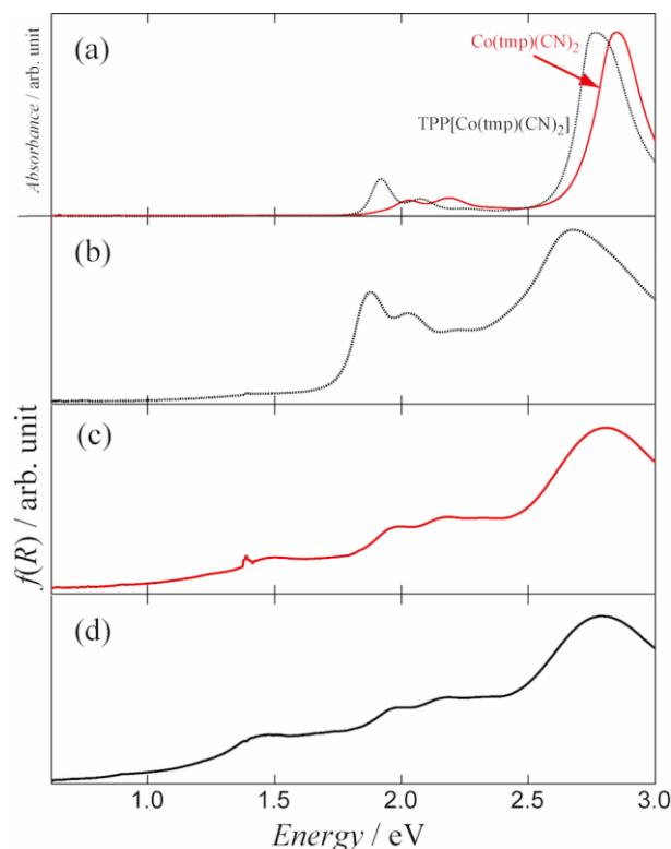
Fig. 10 Vis-NIR spectra of the \text{CH}_3\text{CN} solution of \text{TPP}[\text{Co}(\text{tmp})(\text{CN})_2] and \text{Co}(\text{tmp})(\text{CN})_2 (a), diffuse reflectance spectra of (b) \text{TPP}[\text{Co}(\text{tmp})(\text{CN})_2] \cdot 1/2(\text{acetone}) \cdot \text{H}_2\text{O} , (c) \text{Co}(\text{tmp})(\text{CN})_2 , and (d) \text{Co}(\text{tmp})(\text{CN})_2 \cdot 2\text{CH}_3\text{CN} . The reflectance spectra were converted to the Kubelka-Munk function f(R) .
