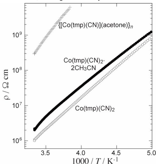
Fig. 11 Temperature dependence of the resistivity of single crystals of \{[\text{Co}(\text{tmp})(\text{CN})](\text{acetone})\}_n , \text{Co}(\text{tmp})(\text{CN})_2 \cdot 2\text{CH}_3\text{CN} , and \text{Co}(\text{tmp})(\text{CN})_2 .
