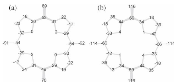
Fig. 9 Comparison of the open shell tmp ligands. Deviation from the least-squares mean plane determined using the core 24 atoms ( d \times 10^2 in Å) for tmp in (a) \text{Co}(\text{tmp})(\text{CN})_2 and (b) \text{Co}(\text{tmp})(\text{CN}) \cdot 2\text{CH}_3\text{CN} .
