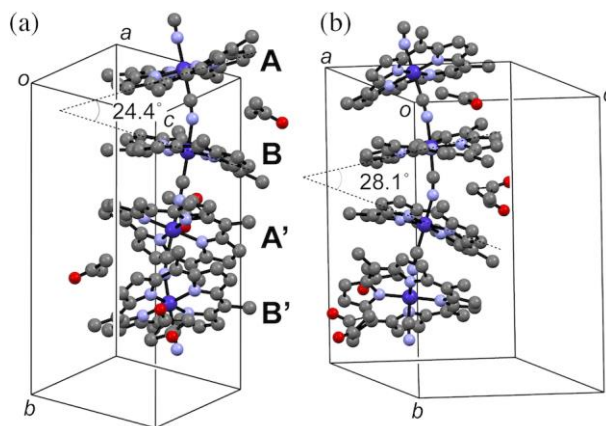
Fig. 3 [\text{Co}(\text{tmp})(\text{CN})]_n polymer chain in \{[\text{Co}(\text{tmp})(\text{CN})](\text{acetone})\}_n ; (a) showing acetone insertion between the rings A and B, and (b) showing acetone insertion between the rings B and A'.
