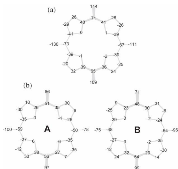
Fig. 4 Comparison of the closed shell tmp ligands. Deviation from the least-squares mean plane determined using the core 24 atoms ( d \times 10^2 in Å) for tmp in (a) \text{TPP}[\text{Co}(\text{tmp})(\text{CN})_2] \cdot 1/2(\text{acetone}) \cdot \text{H}_2\text{O} and (b) \{[\text{Co}(\text{tmp})(\text{CN})](\text{acetone})\}_n .
