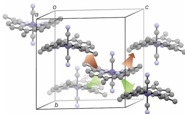
Fig. 5 (a) Perspective view of the unit cell of \text{Co}(\text{tmp})(\text{CN})_2 and (b) perspective view of the unit cell of \text{Co}(\text{tmp})(\text{CN})_2 \cdot 2\text{CH}_3\text{CN} . For clarity, \text{CH}_3\text{CN} molecules are omitted.
