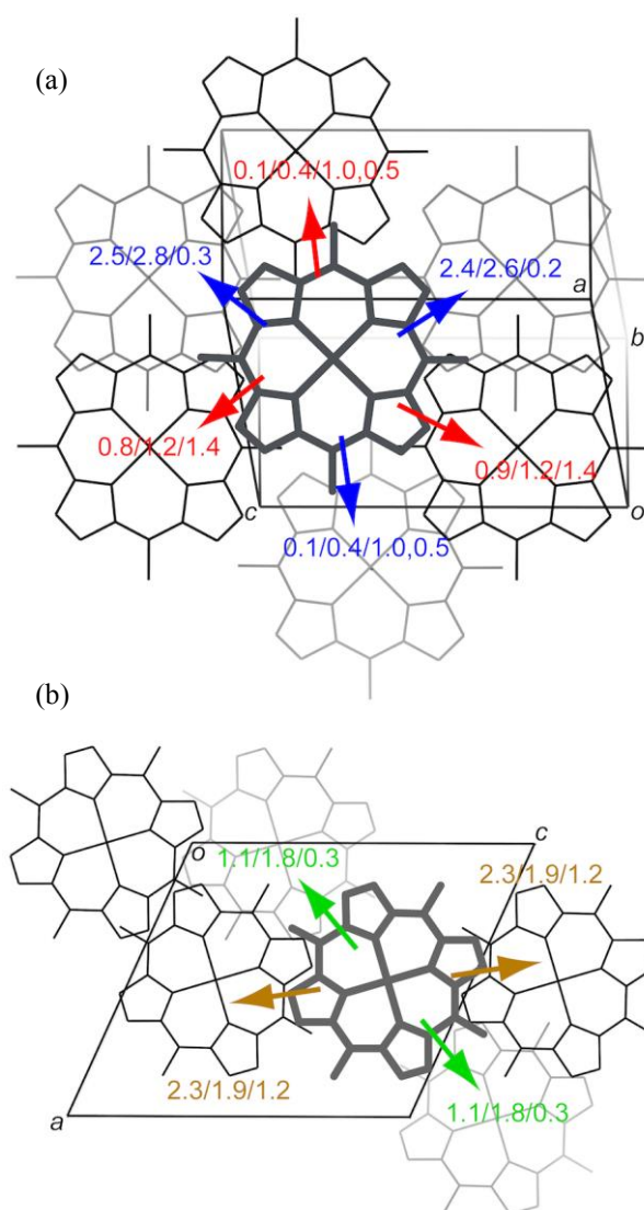
Fig. 8 Overlap integral values (SOMO–SOMO/ HOMO–HOMO/ SOMO–HOMO; all values are \times 10^3 ) (a) between the central radical molecule and six coordinating molecules in \text{Co}(\text{tmp})(\text{CN})_2 (shown in Fig. 5a), and (b) between the central radical molecule and four coordinating molecules in \text{Co}(\text{tmp})(\text{CN})_2 \cdot 2\text{CH}_3\text{CN} (shown in Fig. 5b).
