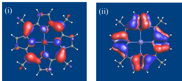
Fig. 7 (a) Energy level diagram and (b) molecular orbitals of (i) SOMO ( a_{2u} ) and (ii) HOMO ( a_{1u} ) of the \text{Co}(\text{tmp})(\text{CN})_2 neutral radical.
