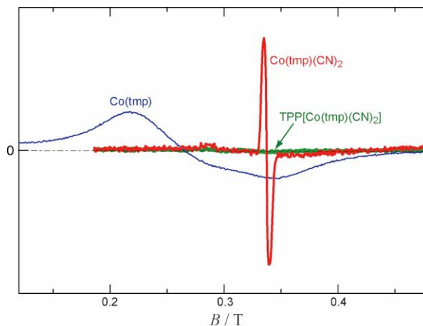
Fig. 6 ESR spectra of \text{Co}(\text{tmp})(\text{CN})_2 , \text{Co}^{\text{II}}(\text{tmp}) , and \text{TPP}[\text{Co}^{\text{III}}(\text{tmp})(\text{CN})_2] \cdot 1/2(\text{acetone}) \cdot \text{H}_2\text{O} . Modulation amplitude and receiver gain for \text{Co}^{\text{II}}(\text{tmp}) were amplified compared with the other two samples.
