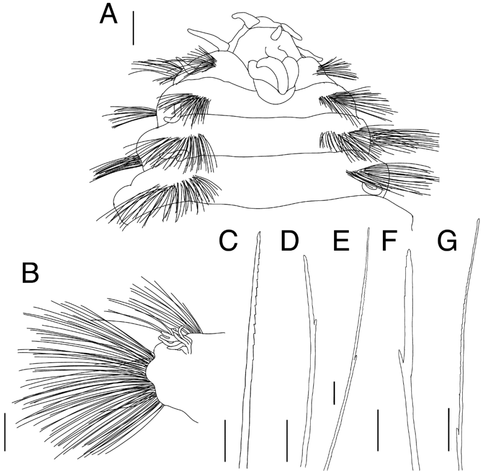
Figure 2. Benthoscolex seisuiae sp. n., holotype (NSMT-Pol H-676). A anterior end, dorsal view B left parapodium of chaetiger 15, posterior view C harpoon notochaeta D bifurcate notochaeta with short tip E bifurcate notochaeta with long tip F bifurcate neurochaeta with short tip G bifurcate neurochaeta with long tip. Scale bars: 1 mm ( A–B ); 100 \mu m ( C–G ).
