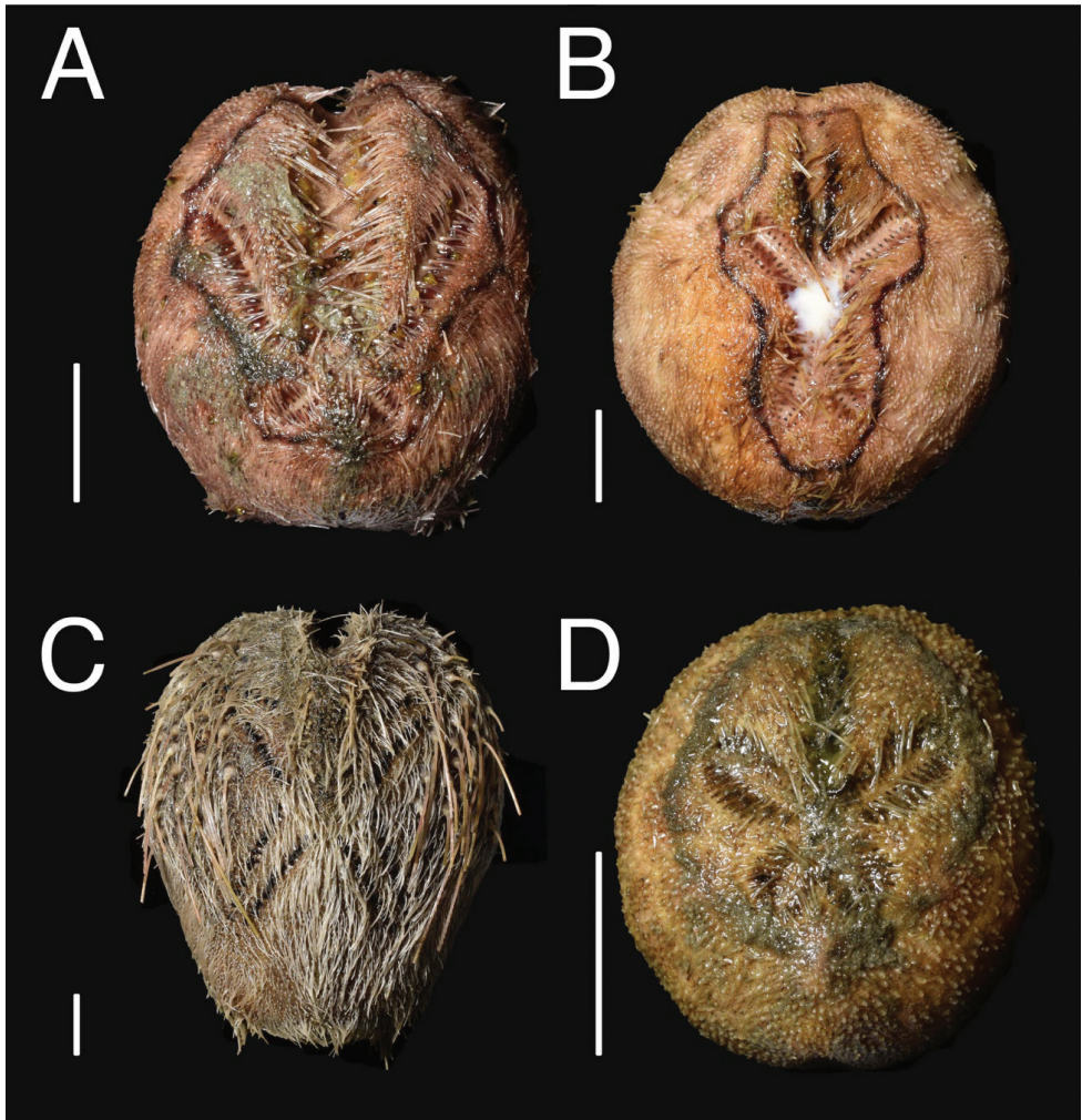
Figure 3. Four of the five irregular sea urchin species that were contained in the same haul with Benthoscolex seisui sp. n., aboral view. A Brisaster latifrons (A. Agassiz, 1898), NSMT E-10723 B Brissopsis luzonica (Gray, 1851), NSMT E-10721 C Lovenia gregalis Alcock, 1893, NSMT E-10719 D Schizaster sp., NSMT E-10725. Scale bars 1 cm.
