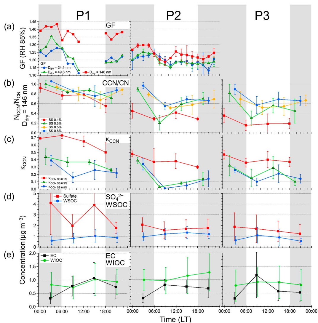
Figure 8. Diurnal profiles of (a) growth factors (GF) at RH of 85%; (b) N_{CCN}/N_{CN} ratios for particles with dry mobility diameter of 146 nm; (c) \kappa_{CCN} under SS of 0.1%, 0.3%, and 0.8%; the mass concentrations of (d) sulfate and water-soluble organic carbon (WSOC); and (e) water-insoluble organic carbon (WIOC) and elemental carbon (EC). Bars indicate \pm 1\sigma (standard deviation) of each average value. Shaded area indicates the nighttime.
