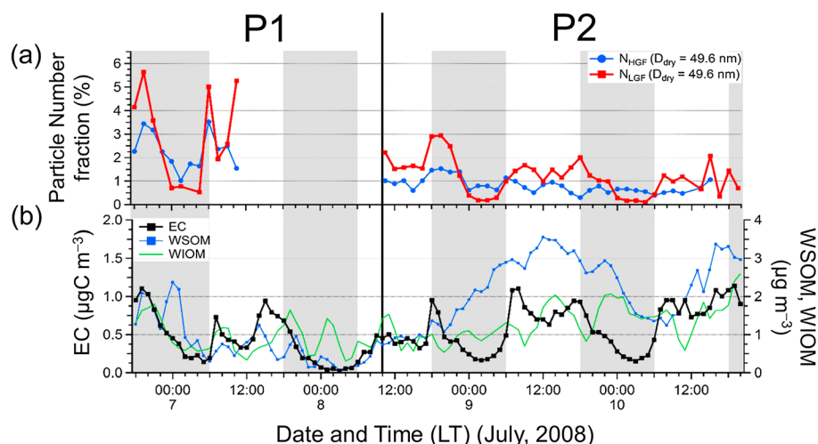
Figure 11. Temporal variations in (a) the particle number fraction for high GF mode ( N_{\text{HGF}} ) and low GF mode ( N_{\text{LGF}} ) particles at D_{\text{dry}} = 49.6 nm, and (b) the mass concentrations of EC, WSOM, and WIOM.
