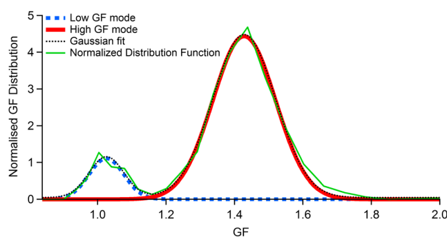
Figure 10. Example of a bimodal GF distribution. For the definition of high GF ( N_{\text{HGF}} ) and low GF ( N_{\text{LGF}} ) modes, see text. The GF distribution is calculated using a multiple Gaussian fit applied on the normalized distribution function. Separation of the modes was made by cluster analysis using the program IGOR Pro.
