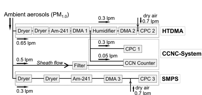
Figure 2. Schematic of the experimental setup for the HTDMA, CCNC, and SMPS.
