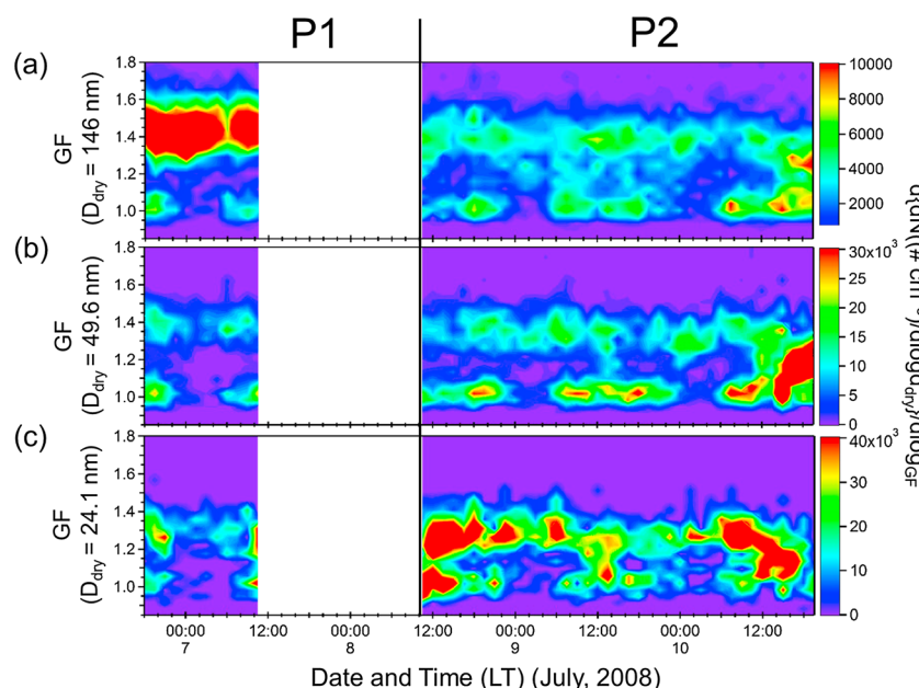
Figure 6. Temporal variations in the particle number concentrations as a function of the growth factor (GF) at D_{\text{dry}} of (a) 146 nm, (b) 49.6 nm, and (c) 24.1 nm.
