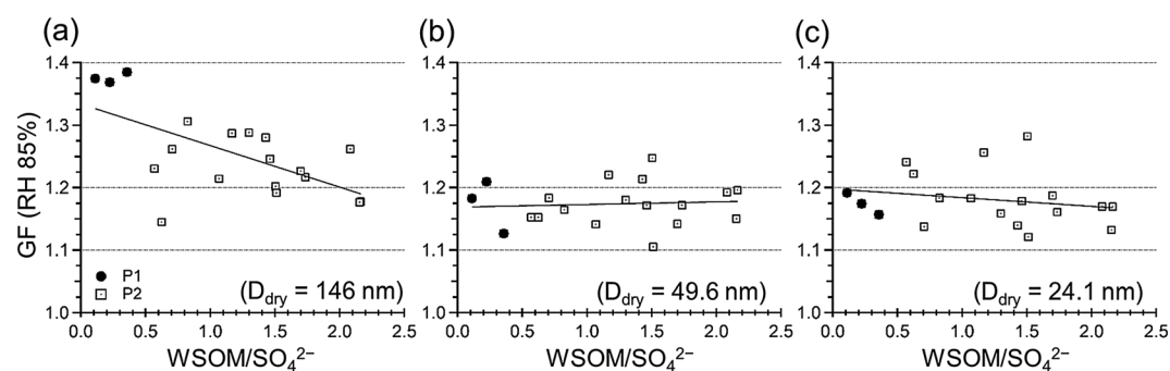
Figure 12. Scatterplot of hygroscopic GF versus ratio of the WSOM to sulfate at D_{\text{dry}} of (a) 146 nm, (b) 49.6 nm, and (c) 24.1 nm. Data during P1 and P2 are indicated by solid circles and open squares, respectively.
