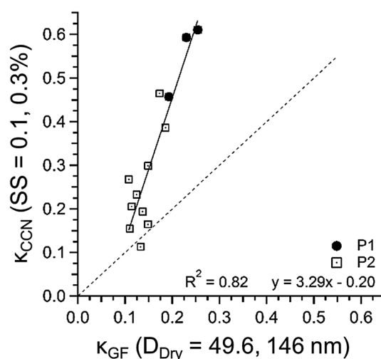
Figure 7. Scatterplot of \kappa_{\text{CCN}} versus \kappa_{\text{GF}} . The average \kappa_{\text{GF}} at D_{\text{dry}} of 49 and 146 nm are compared with the average \kappa_{\text{CCN}} at similar D_{\text{act}} under SS of 0.1% and 0.3%. The data obtained during P1 and P2 are indicated by solid circles and open squares, respectively.
