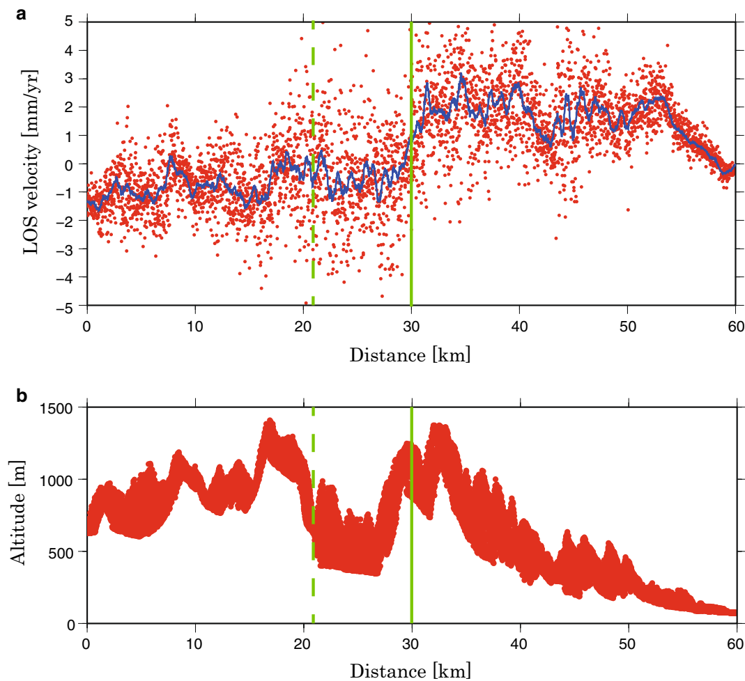
Fig. 8 Profiles of a LOS velocities and b altitudes along AA' in Fig. 7. Blue line indicates 30 points running average. Green solid and broken lines at ~30 km and ~21 km along the horizontal axis indicate the location of the Ushikubi and Atotsugawa faults, respectively
