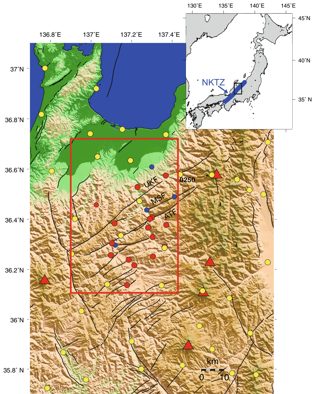
Fig. 1 Shaded relief map of the Atotsugawa fault system and surrounding region. The black lines indicate active faults. The Atotsugawa fault (ATF), Mozumi–Sukenobu fault (MSF), and Ushikubi fault (UKF) comprise the Atotsugawa fault system. Yellow circles indicate GEONET stations. Red circles indicate our GNSS stations used for correcting the interferograms. Blue circles indicate our GNSS stations not used for corrections. GEONET station 0250 was used as the reference. The red frame indicates the area shown in Figs. 5 and 7. Active volcanoes appear as triangles. The inset shows the location of the study area (black frame) within the Japan arc. The blue line indicates the Niigata–Kobe Tectonic Zone (NKTZ)
