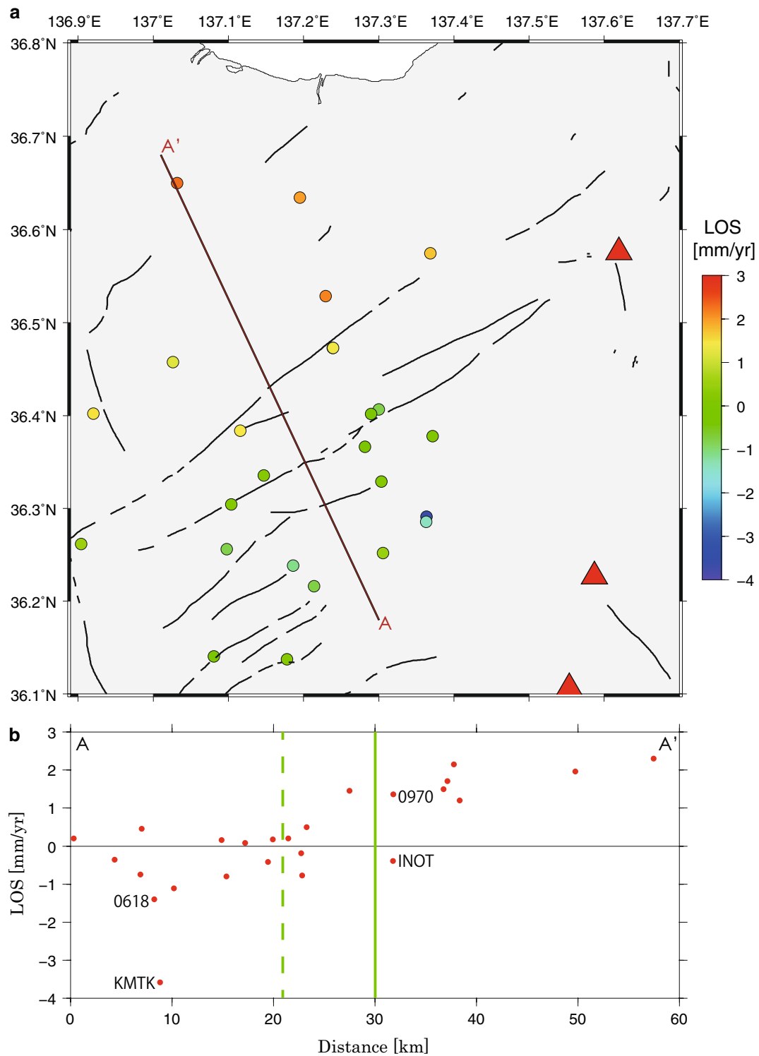
Fig. 9 a LOS velocities calculated from GNSS data. Red triangles indicate active volcanoes. b One-dimensional profile of the GNSS-derived LOS velocities. The profile is indicated by the red line (AA') in a , which is the same as AA' in Fig. 7. Green solid and broken lines at ~30 and ~21 km along the horizontal axis indicate the locations of the Ushikubi and Atotsugawa faults, respectively
