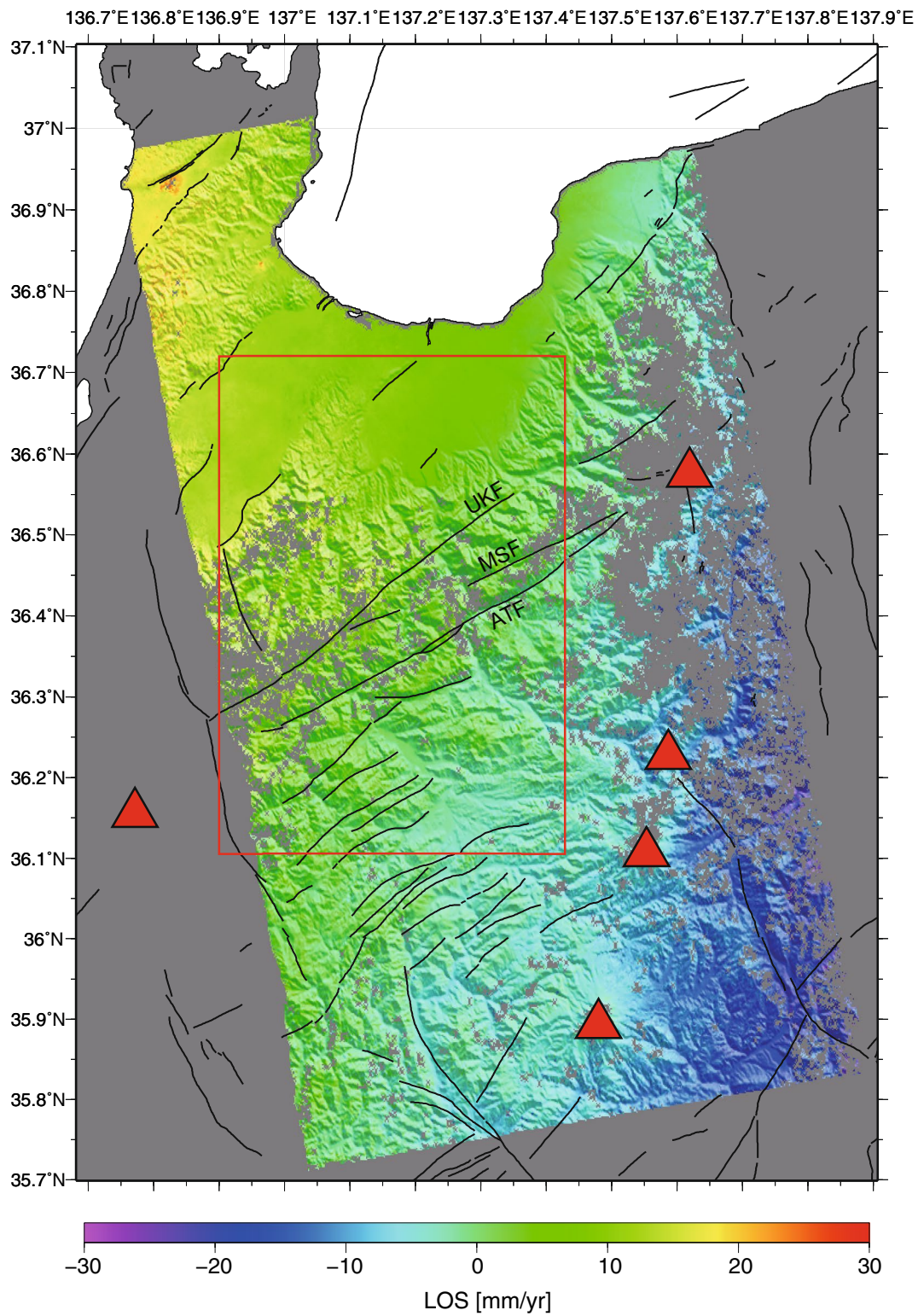
Fig. 3 Mean velocity field in and around the Atotsugawa fault system calculated using the InSAR time-series analysis. Note that color scale ranges from -30 to 30 mm/yr. The red frame indicates the area shown in Figs. 5 and 7. Triangles indicate active volcanoes. Black lines represent active faults
