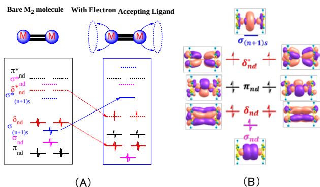
Fig. 3 (A) Orbital interaction between W_2 and two benzene ligands. (B) the MOs of C_6H_6(W_2)C_6H_6 with D_{6h} symmetry.
