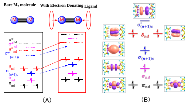
Fig. 4 (A) Orbital interactions between electron-donating ligands and M_2 moiety. (B) The dominant electron configuration of the O_4(W_2)O_4 complex.
