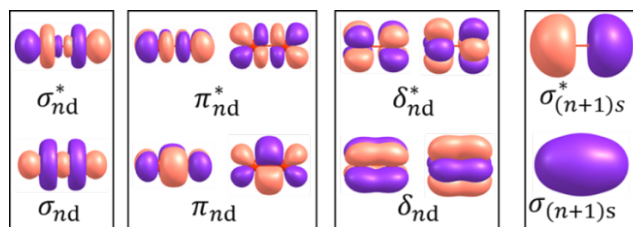
Fig. 1 Molecular orbitals contributing to sextuple bond in transition metal element.
