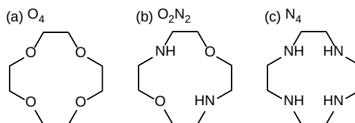
Scheme 1. Structures of (a) 12-crown-4 ether ( O_4 ), (b) 1,7-diaza-12-crown-4 ether ( O_2N_2 ), and (c) 1,4,7,10-tetraza-12-crown-4 ether ( N_4 )
