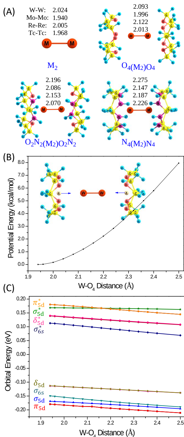
Fig. 5 (A) Structures of the bare M_2 and the dinuclear complexes. The numbers are the metal-metal bond lengths in Å. (B) Potential energy curve of the W- O_4 coordination in S_0 state. (C) Change in orbital energies against W- O_4 distance. The W- O_4 distance is defined as that between W and X (the center of the four O atoms). Calculations were performed with DFT; see section S1 in ESI for computational details.
