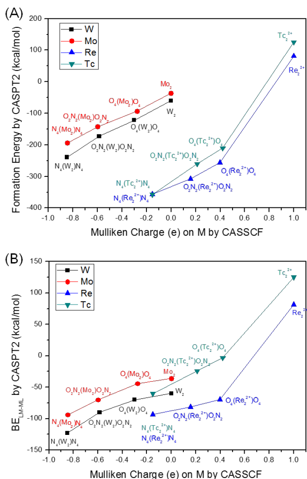
Fig. 8 The correlation of (A) formation energy and (B) BE_{LM-ML} with calculated atomic charge of transition metal.
