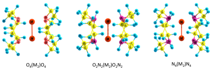
Fig. 6. The structures of the M_2 -side O_4(M_2)O_4 , O_2N_2(M_2)O_2N_2 , and N_4(M_2)N_4 complexes.
