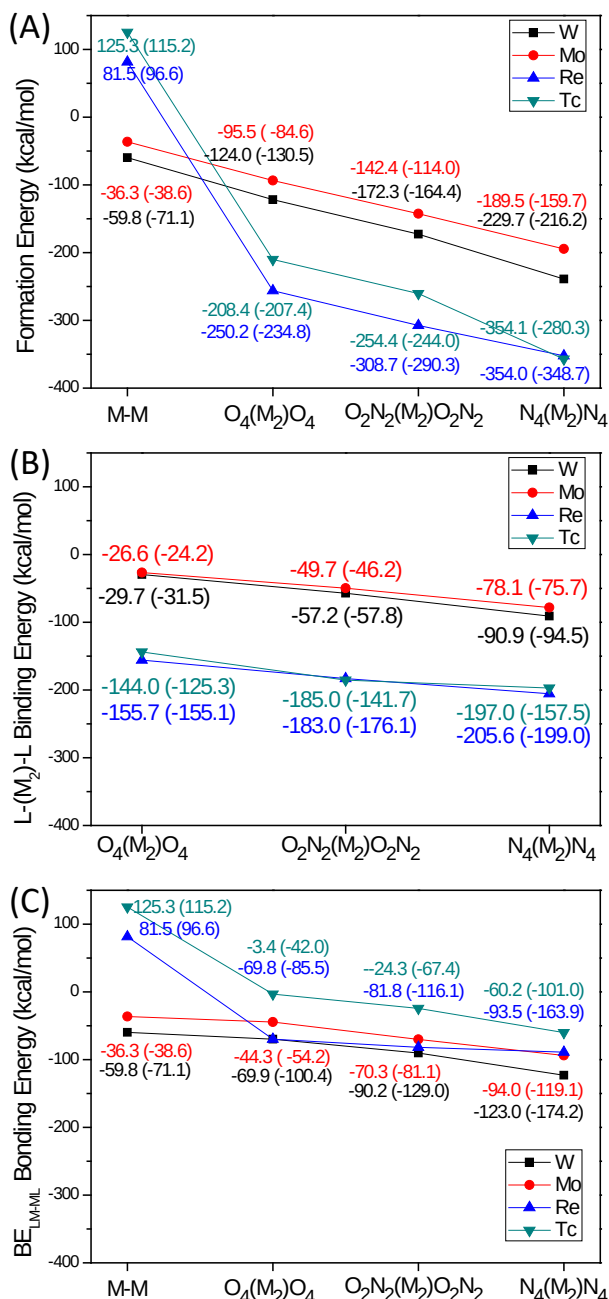
Fig. 7 Formation energy (eq. 2) and binding energy (eqs. 3 and 4) calculated with CASPT2 method. The values in parentheses are calculated by the DFT method. The negative values of the formation energy and the binding energy correspond to the exothermicity. (A)
