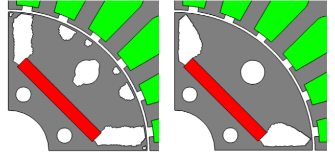
T_{ave} = 2.37\text{Nm} , T_{rip} = 0.28 (a) Gaussian basis function T_{ave} = 2.27\text{Nm} , T_{rip} = 0.21 (b) Polygon morphing Fig.6 Optimized shapes of IPM motor
