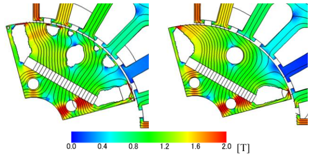
(a) Gaussian basis function (b) Polygon morphing Fig.7 Magnetic induction and flux lines in optimized IPM motors
