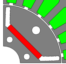
(b) Base model of IPM represented by \phi
