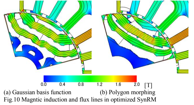
Fig.10 Magnetic induction and flux lines in optimized SynRM
