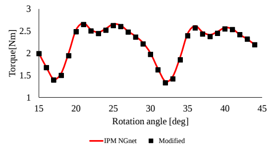
Fig.13 Effect of smoothing
