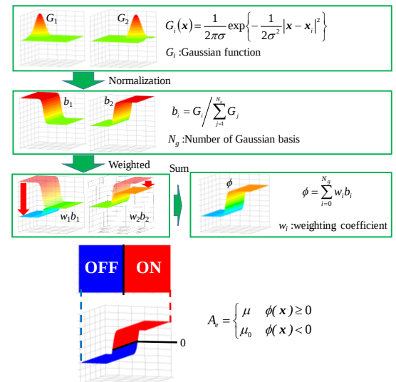
Fig.1 On/off method using normalized Gaussians
