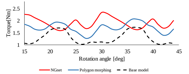
Fig.11 Torque waveforms of synchronous reluctance motor
