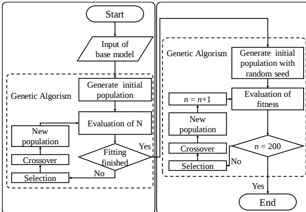
Fig.2 Flow diagram of present method
