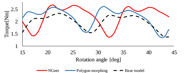
Fig.8 Torque waveforms of IPM motor
