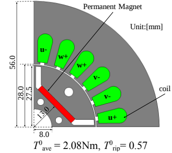
(a) Base model of IPM motor
