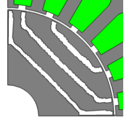
(c) Base model of SynRM represented by \phi
