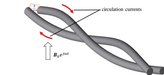
Fig.7. Circulation currents in a pair of wires.
