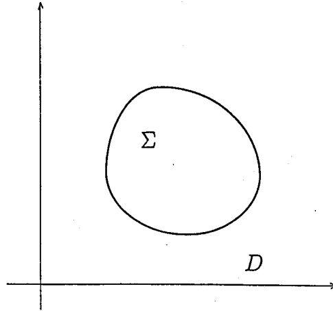
Figure 2: \overline{\Sigma} \subset D
