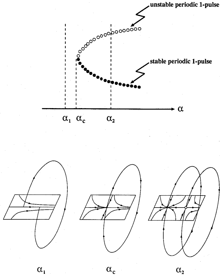
Figure 3.11: Dynamics near the limiting point; Even after the event of the saddle-node bifurcation, there still remains an oscillatory motion at \alpha = \alpha_1 . The temporary oscillatory motion lasts longer and longer, when \alpha_1 approaches \alpha_c .
