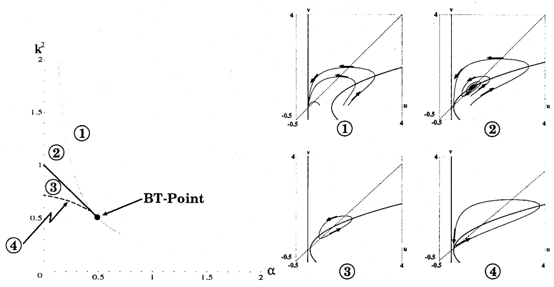
Figure 2.3: Unfolding of Bogdanov-Takens point.
