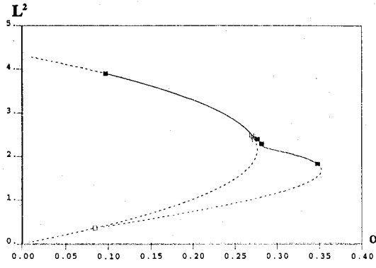
Figure 3.6: Emergence of Turing branch of 2-mode ( d = 0.53, n = 8 ).
