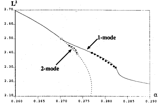
Figure 3.6: Emergence of Turing branch of 2-mode ( d = 0.53, n = 8 ).
