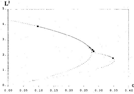
Figure 3.7: Interaction of Turing branches ( d = 0.52, n = 8 ).
