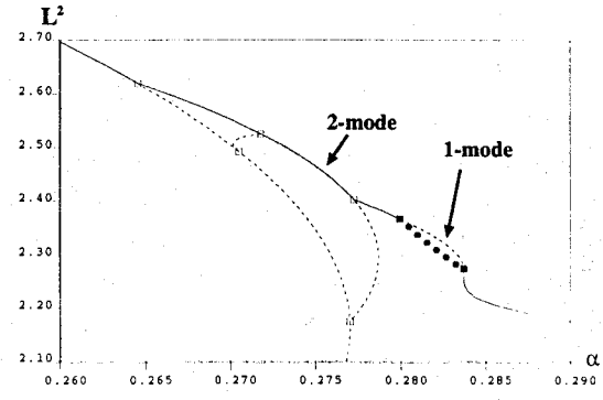
Figure 3.7: Interaction of Turing branches ( d = 0.52, n = 8 ).
