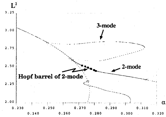
Figure 3.8: Emergence of Hopf barrel on Turing branch of 2-mode ( d = 0.2, n = 8 ).
