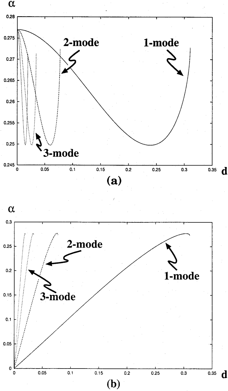
Figure 3.1: Turing bifurcation curves in (d, \alpha) -space ( n = 1, 2, \dots, 4 ) for PDE model on (0, \pi) with k = 0.95 ; (a) (resp.(b)) shows the location of bifurcation points on the upper (resp. lower) branch of the saddle-node branch. Note that the bifurcation points on the upper branch are concentrated near the saddle-node point \alpha_c = 0.277 (the difference between the maximum and the minimum values of 1-mode is about 0.026), and the smaller d , the larger mode-number primarily emerges as \alpha increases.
