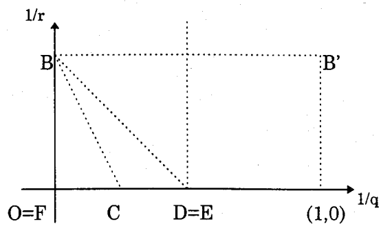
Figure 3. n = 2 .
