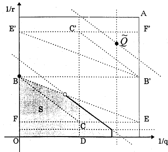
Figure 5. Corollary 2.1 ( n > 3 ).
