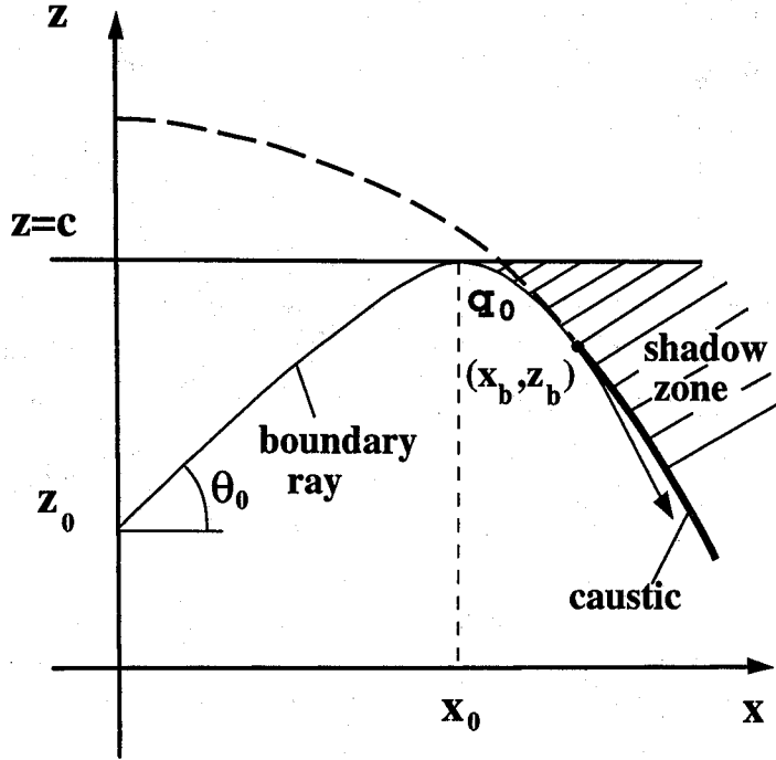
Figure 3. Boundary ray and shadow zone
