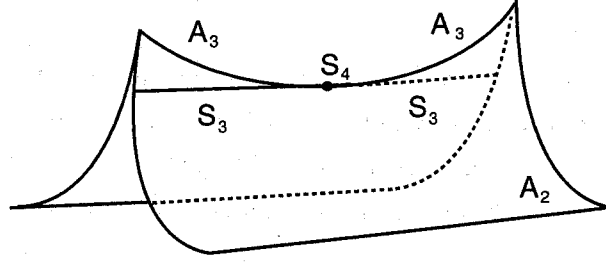
Figure 1: S_4 -caustic
