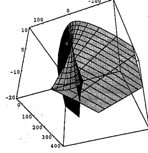
swallowtail
