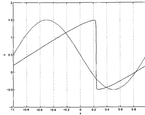
Figure 13: Numerical solution (WENO5-LLF) to the Burgers Equation with shifted sine wave as initial data. We plotted the zero level set at time t = 0 and 0.5 .
