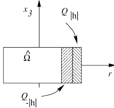
Fig. 2. Sets Q_h .
