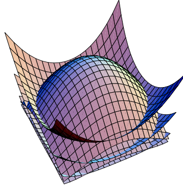
The phase portrait \{\pi \circ f(\mu^{-1}(c))\}_{c \in \mathbb{R}} of DA_2^0 for n=2 .
