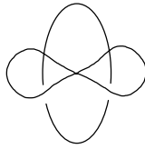
Figure 2: The interesting singular fibre III^{13} in Theorem 1.1
