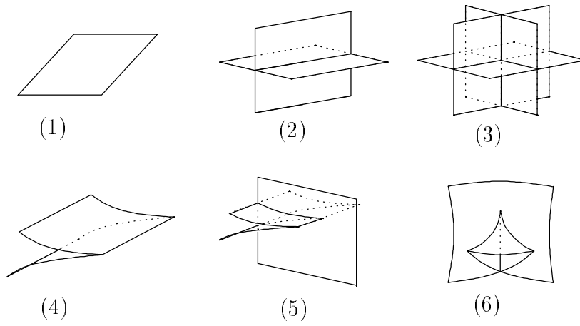
Figure 3: Multi-singularities of f|_{S(f)}
