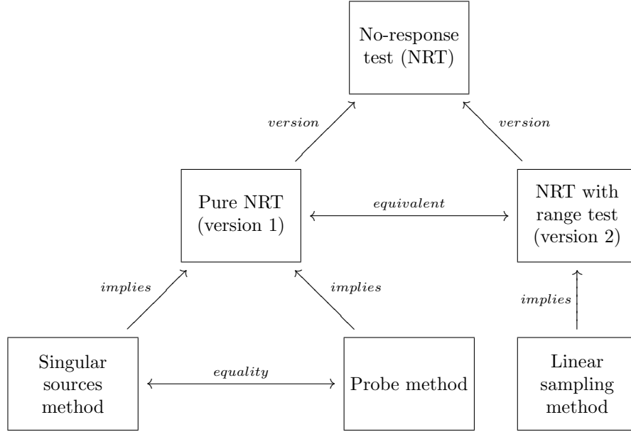
Figure 1: The Diagramm shows the relation between the two versions of the no-response test and several non-iterative methods for the inverse scattering theory.
