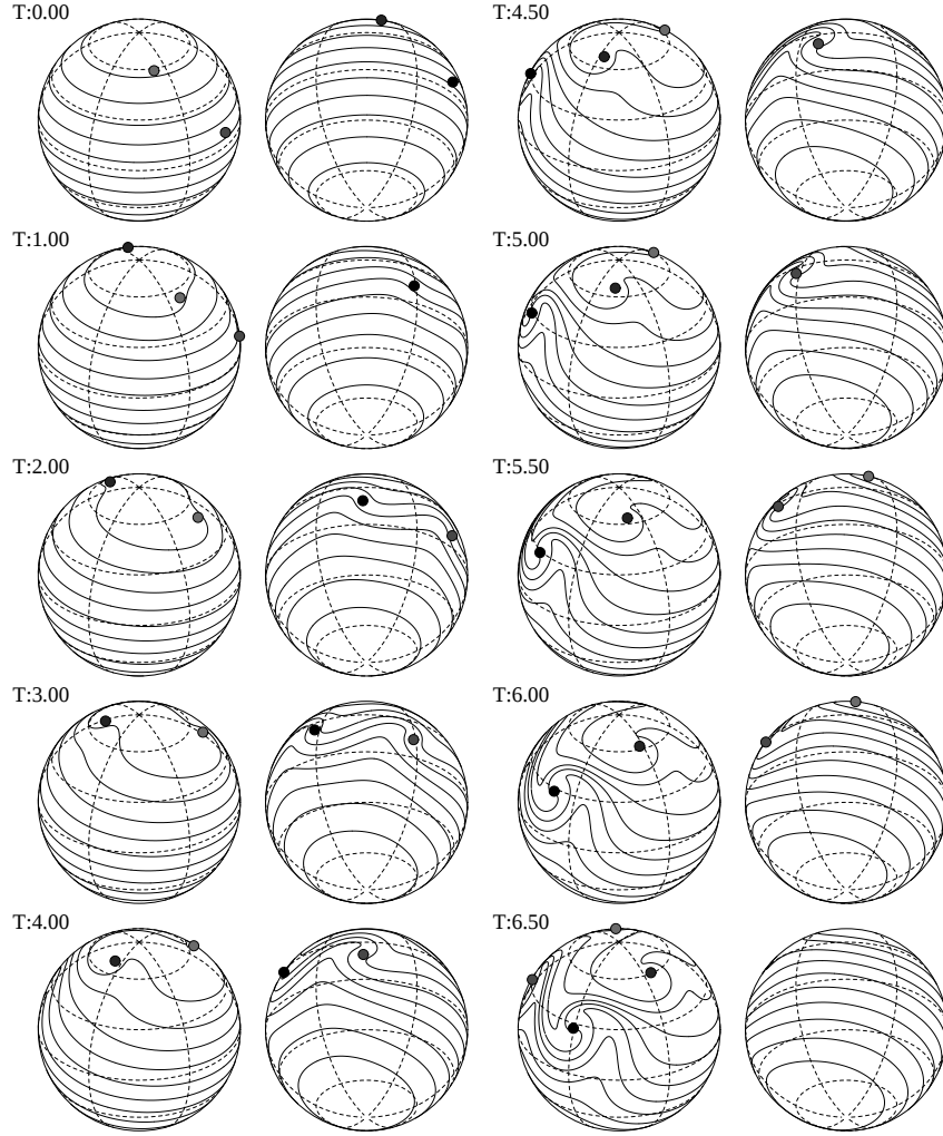
Figure 2. Evolution of ring configuration and contours with N = 4 and M = 10 and frequency ratio 4:1. Orientation \gamma = \pi/4 and \theta_0 = \pi/4 . T = 0.0 - 6.5 in dimensionless units.
