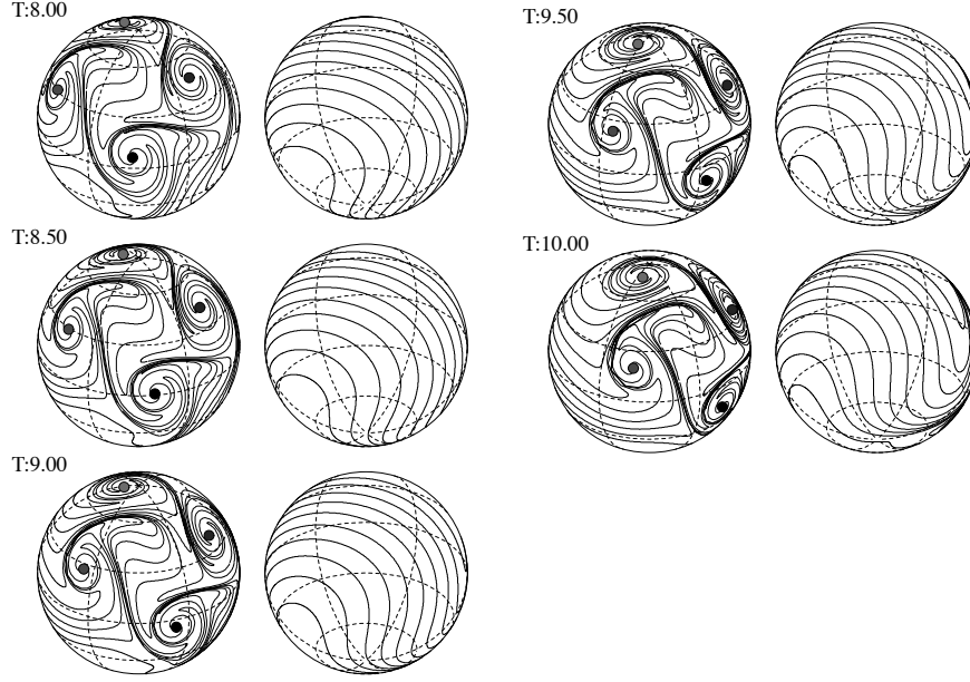
Figure 11. Same as previous figure but with T = 8.0 - 10.0 in dimensionless units. Note the wrapping of the contours around the point vortices effectively increases their strength. The ring stays relatively intact throughout the evolution.
