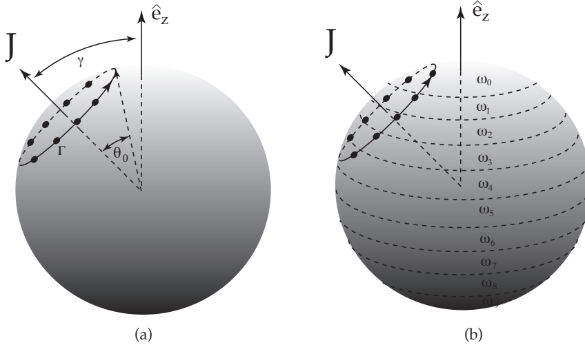
Figure 1. Initial configuration with N equal strength point vortices ( \Gamma ) evenly spaced around a spherical cap which gives rise to the \mathbf{J} -vector as shown. (a) The size of the spherical cap is characterized by the base half-angle \theta_0 , while the orientation with respect to the axis of rotation is characterized by angle \gamma . (b) 10 constant vorticity strips \omega_n = \text{const.} with 9 contours that require tracking. The constant values \omega_n are chosen so that they approximate the vorticity distribution corresponding to solid-body rotation around the z -axis. See text for more details.
