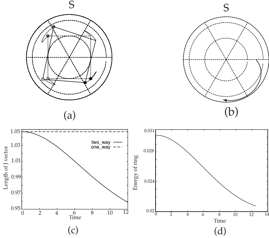
Figure 9. (a) Evolution of point vortices in a frame of reference rotating with the background frequency of the one-way coupled model with a frequency ratio -4:1. In contrast to figure 4, the original rotational direction of the ring is never regained and the ring loses its coherence much more quickly. (b) Evolution of the tip of the center of vorticity vector J associated with the ring. Note that it still rotates towards the North Pole. (c) Evolution of the length of the center of vorticity vector \|J\| which decreases as the contours wrap around the vortex centers. (d) The Hamiltonian is no longer conserved when the ring is coupled to the background. In this case, since the ring is counter-rotating with the background, it is losing energy to it.
