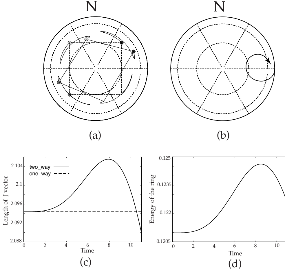
Figure 12. (a) Evolution of point vortices in a frame of reference rotating with the background frequency of the one-way coupled model with a frequency ratio 2:1 and \gamma = \pi/2 . For this symmetric case, the ring briefly reverses direction, but as the strength of the vortices increases, it regains its original rotational direction as in the previously discussed co-rotating cases. (b) Evolution of the tip of the center of vorticity vector J associated with the ring. Note that it spirals up towards the North Pole. (c) Evolution of the length of the center of vorticity vector \|J\| which is constant in the one-way coupled model but not when the ring is coupled to the background flow. In this case, as the vortices increase their strength by wrapping themselves in the contours, the length of J evolves in a more complex manner than either the co-rotating or counter-rotating cases discussed previously. Initially its length increases but then reverses direction. (d) Evolution of the Hamiltonian energy of the ring which achieves a local maximum at roughly the same time as \|J\| .
