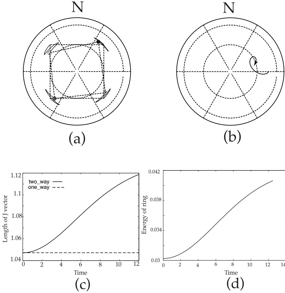
Figure 4. (a) Evolution of point vortices in a frame of reference rotating with the background frequency of the one-way coupled model with a frequency ratio 4:1. Note that the ring briefly reverses direction, but as the strength of the vortices increases, it regains its original rotational direction and the ring remains relatively intact. (b) Evolution of the tip of the center of vorticity vector J associated with the ring. Note that it rotates up towards the North Pole. (c) Evolution of the length of the center of vorticity vector \|J\| which is constant in the one-way coupled model but not when the ring is coupled to the background flow. In this case, as the vortices increase their strength by wrapping themselves in the contours, the length of J increases. (d) The Hamiltonian is no longer conserved when the ring is coupled to the background. In this case, since the ring is co-rotating with the background, it is gaining energy from it.
