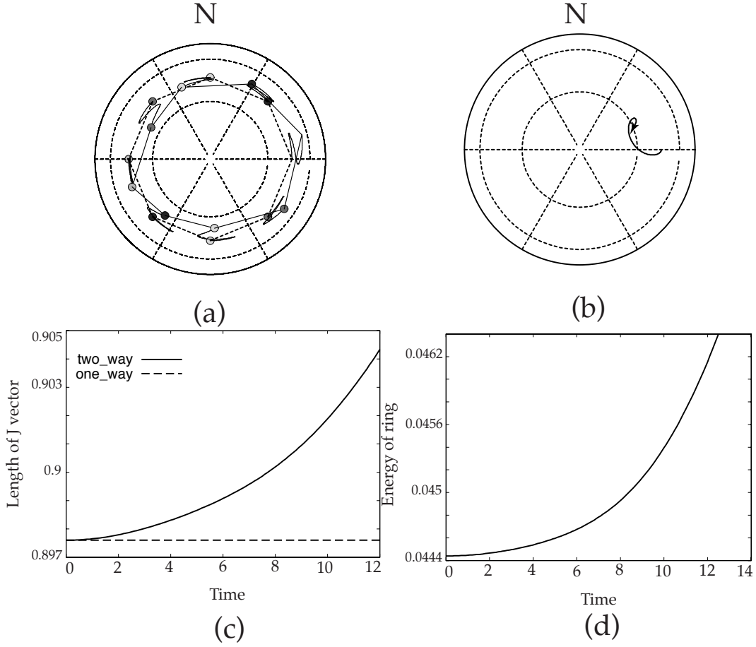
Figure 7. Same parameters as figure 4 but with N = 8 . The conclusions are robust with respect to changes in N .
