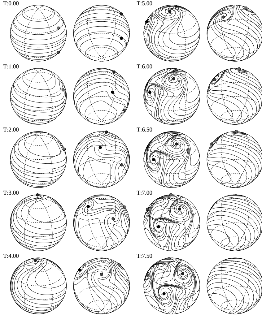
Figure 10. Evolution of ring configuration and contours with N = 4 and M = 10 and frequency ratio 2:1. Orientation \gamma = \pi/2 and \theta_0 = \pi/4 . T = 0.0 - 7.5 in dimensionless units. Note that for this orientation, if the sign of \Gamma is reversed, the evolution of the system will be identical but in the opposite hemisphere.
