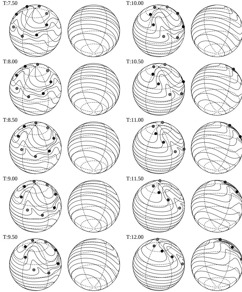
Figure 6. Same as previous figure but with T = 7.5 - 12.0 in dimensionless units. Note the wrapping of the contours around the point vortices effectively increases their strength. The ring stays relatively intact throughout the evolution.
