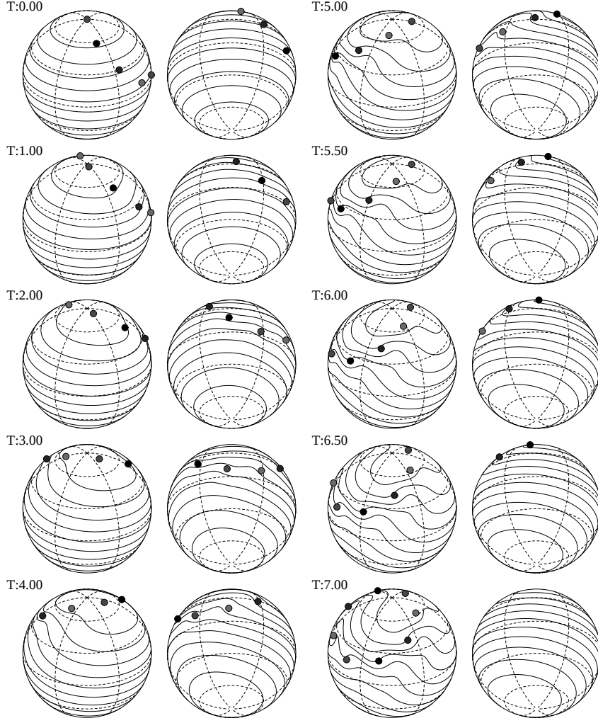
Figure 5. Evolution of ring configuration and contours with N = 8 and M = 10 and frequency ratio 4:1. Orientation \gamma = \pi/4 and \theta_0 = \pi/4 . T = 0.0 - 7.0 in dimensionless units.
