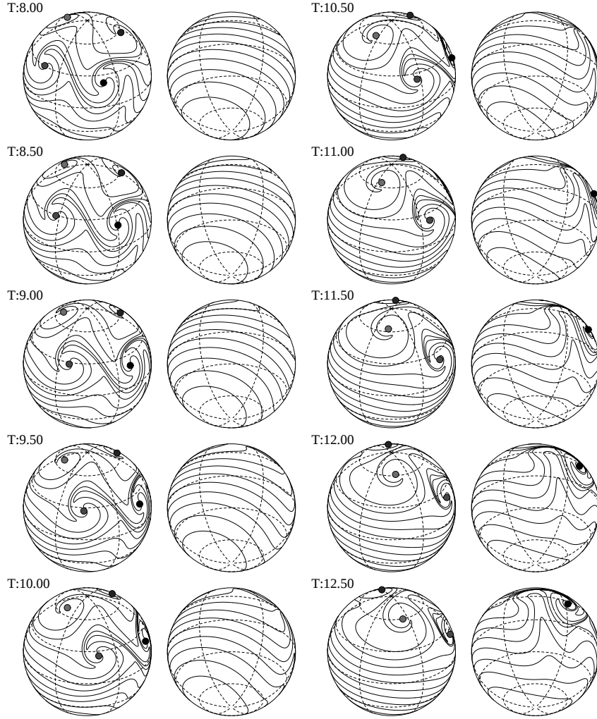
Figure 3. Same as previous figure but with T = 8.0 - 12.5 in dimensionless units. Note the wrapping of the contours around the point vortices effectively increases their strength with respect to the background. The ring stays relatively intact throughout the evolution.
