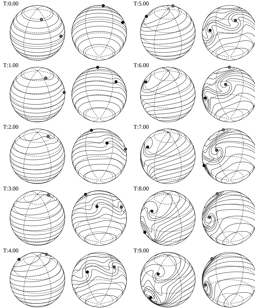
Figure 8. Evolution of ring configuration and contours with N = 4 and M = 10 and frequency ratio -4:1. Orientation \gamma = \pi/4 and \theta_0 = \pi/4 . T = 0.0 - 9.0 in dimensionless units. In contrast to the co-rotating case, the wrapping of the contours around the point vortices causes their strength to decrease (in absolute magnitude) relative to the background.
