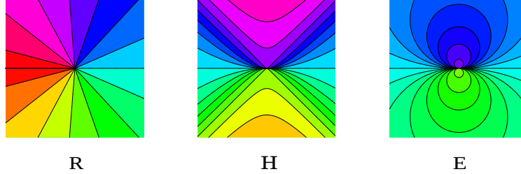
Figure 1: phase singularities
