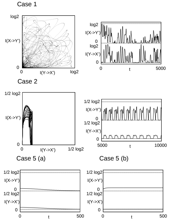
FIG. 3: (Top) Case 1: Aperiodic information flow. (Middle) Case 2: Periodic switching among aperiodic information flow. (Bottom) Case 5: (a) stationary information flow I(Y \rightarrow X' : X, Y) = I(X \rightarrow Y' : X, Y) = 0 . (b) stationary information flow I(Y \rightarrow X' : X, Y) = 0.00305395 and I(X \rightarrow Y' : X, Y) = 0.06023025 .
