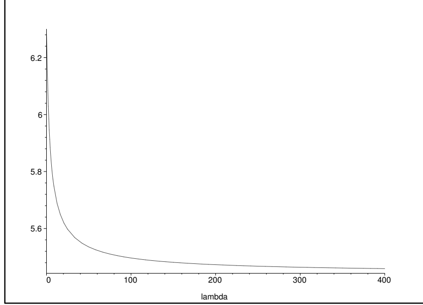
Figure 2. The variation of Riemannian length of the indicatrix for the metric given in Example 2.
