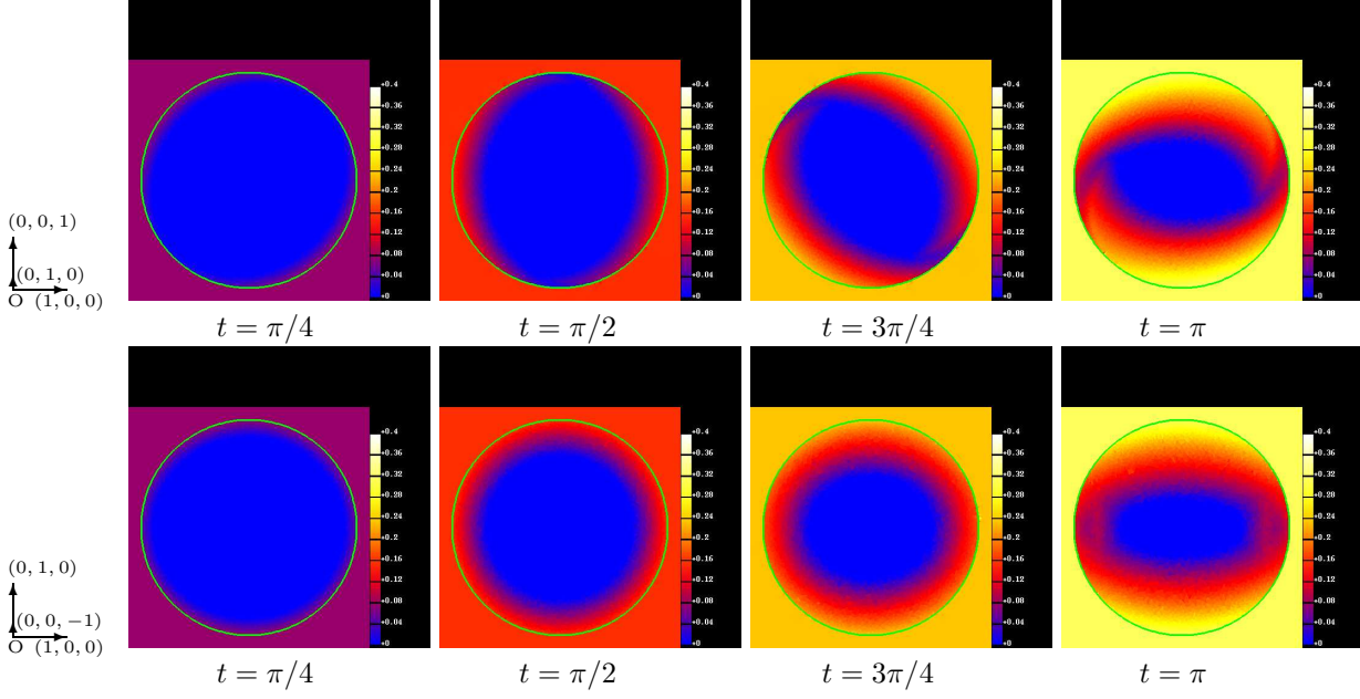
FIGURE 8. The magnitude of the magnetic flux \mathcal{B} on the cross-sections of \Omega cut by the plane y = 0 (first row), by the plane z = 0 (second row) for Case 1.
