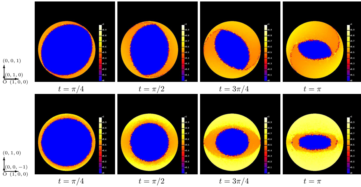
FIGURE 5. The magnitude of the electric current \mathcal{J} on the cross-sections of \Omega_s cut by the plane y = 0 (first row), by the plane z = 0 (second row) for Case 1.
