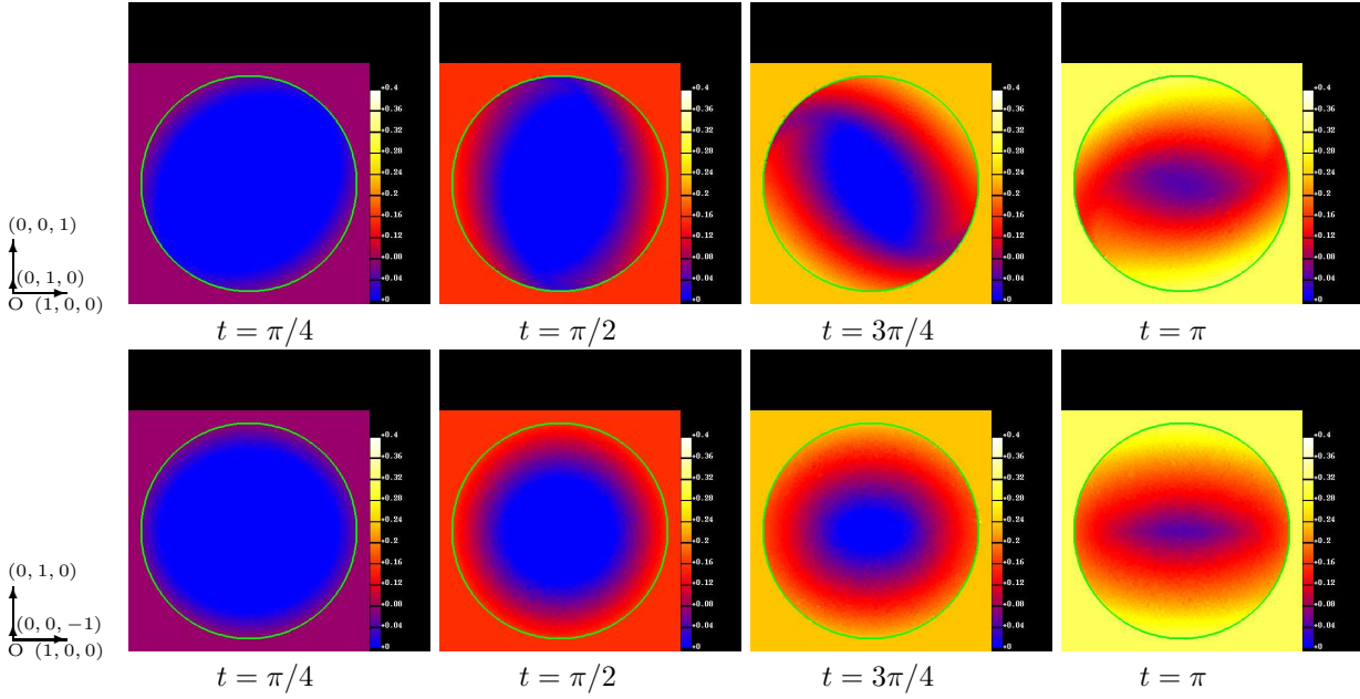
FIGURE 9. The magnitude of the magnetic flux \mathcal{B} on the cross-sections of \Omega cut by the plane y = 0 (first row), by the plane z = 0 (second row) for Case 2.
