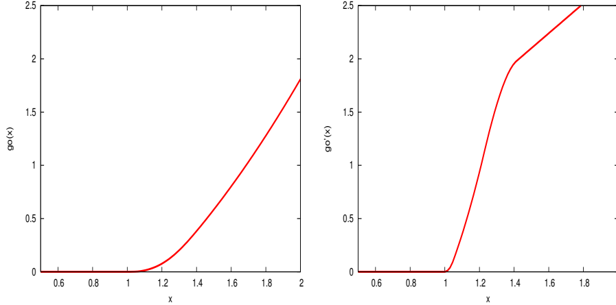
FIGURE 2. The graph of g_0(x) (left) and the graph of g'_0(x) (right).
