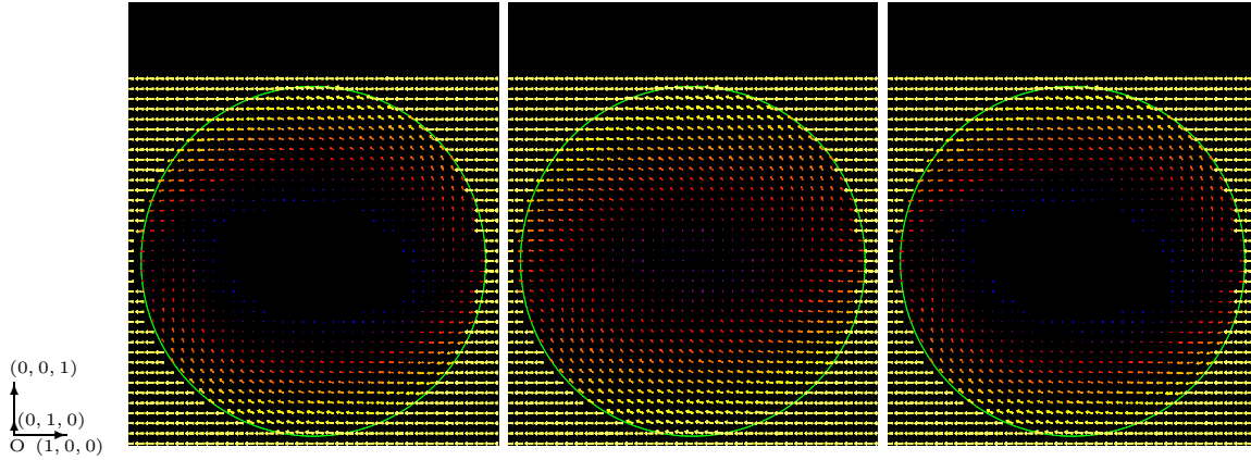
FIGURE 11. The direction of the magnetic flux \mathcal{B} on the cross-section of \Omega cut by the plane y = 0 at t = \pi : Case 1 (left), Case 2 (centre), Case 3 (right). The colour scale is same as that of Figures 8-10 at t = \pi .
