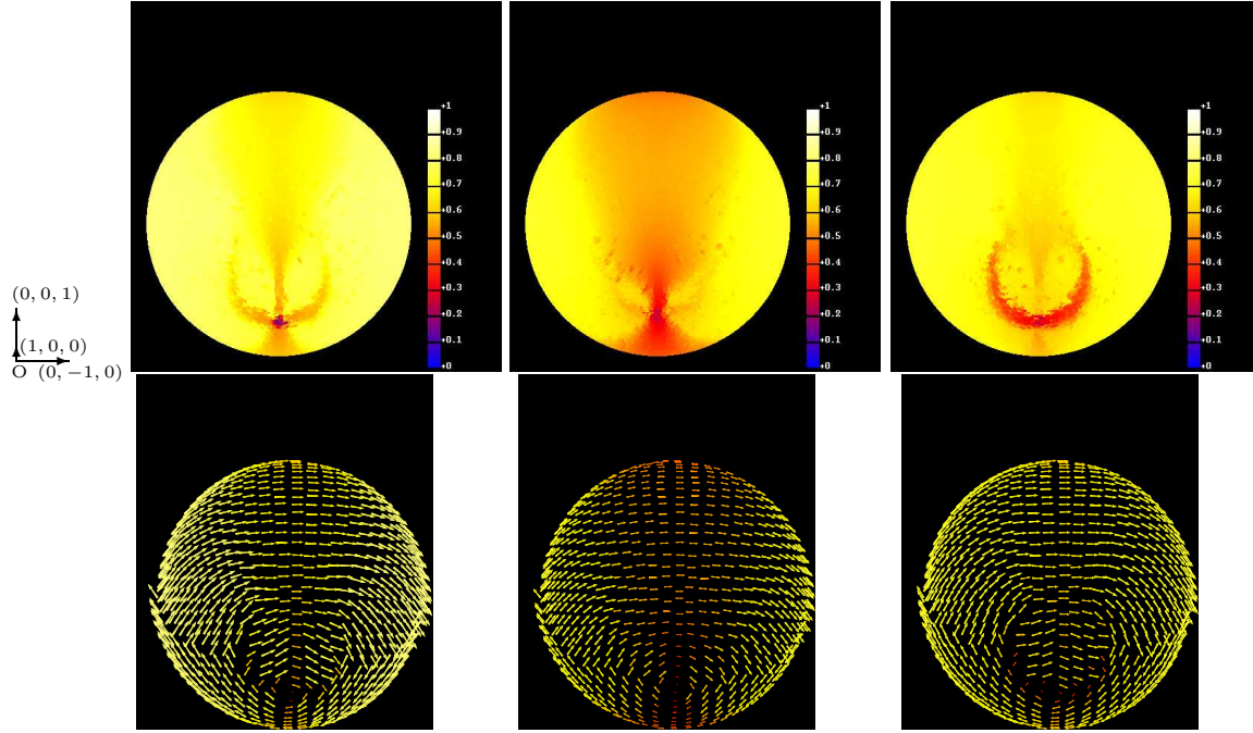
FIGURE 4. The electric current \mathcal{J} on the surface \partial\Omega_s at t = \pi . The first row and the second row show the magnitude and the direction, respectively: Case 1 (left), Case 2 (centre), Case 3 (right).
