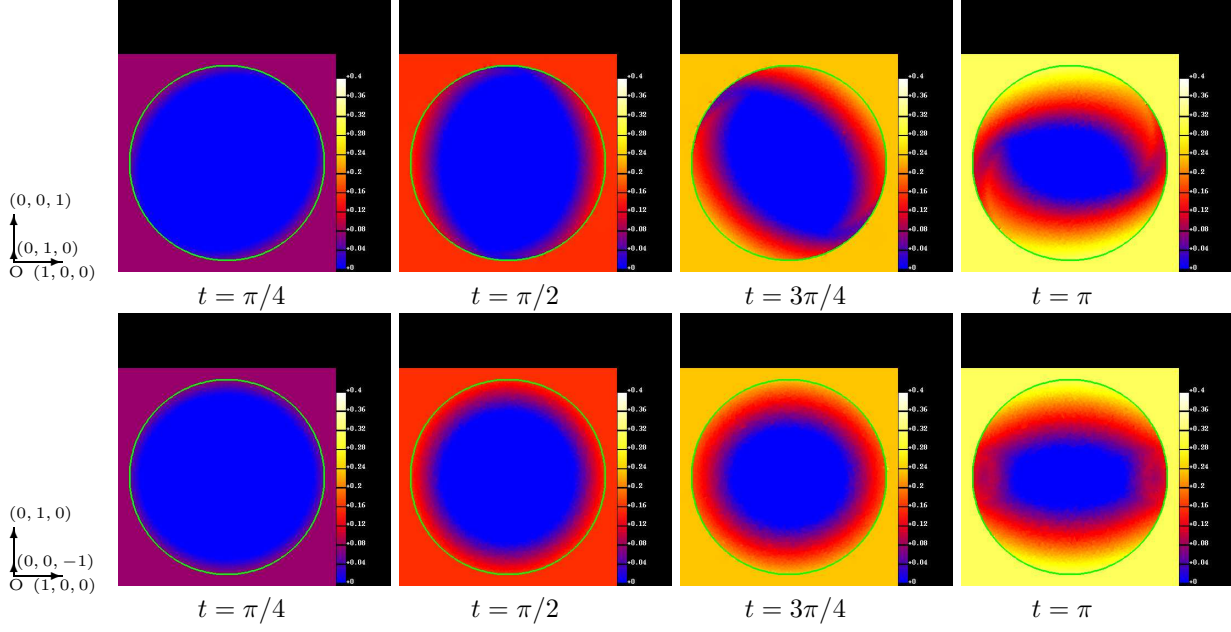
FIGURE 10. The magnitude of the magnetic flux \mathcal{B} on the cross-sections of \Omega cut by the plane y = 0 (first row), by the plane z = 0 (second row) for Case 3.
