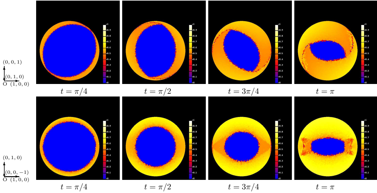
FIGURE 7. The magnitude of the electric current \mathcal{J} on the cross-sections of \Omega cut by the plane y = 0 (first row), by the plane z = 0 (second row) for Case 3.
