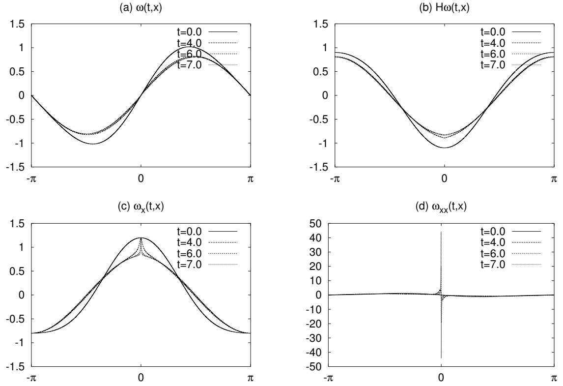
Figure 1: Numerical solution of the equation (1) for the initial data (8) with \epsilon = 0.1 . (a) \omega(t, x) , (b) H\omega(t, x) , (c) \omega_x(t, x) and (d) \omega_{xx}(t, x)
