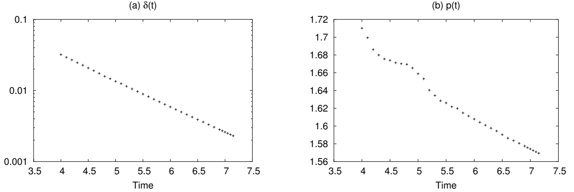
Figure 3: (a) Log plot of \delta(t) , (b) plot of p(t) in the Ansatz (9) obtained from the numerical solution.
