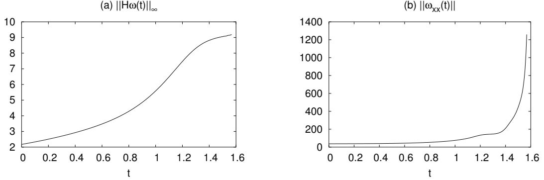
Figure 7: Graphs of \|H\omega(t)\|_\infty (a) and \|\omega_{xx}(t)\| (b). The initial value is \omega(0, x) = 0.2 \cos x + \sin 4x + \sin 7x .
