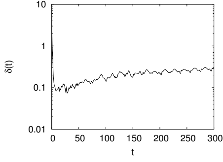
Figure 8. Time evolution of the analyticity strip \delta(t) up to t = 300 for \alpha = 0.4 in a semi-log plot.
