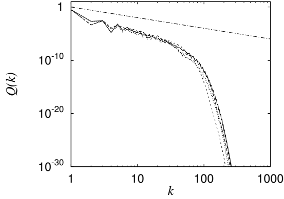
Figure 5. Time evolution of the spectra of active scalar at t = 70 (solid), 80 (dashed), 90 (dotted), and 100 (short-sashed). The straight line has a slope of -2 .
