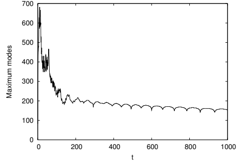
Figure 29. Time evolution of the maximally excited number up to t = 1000 . for Case 2 with \alpha = 0.4 .
