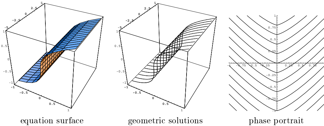
Figure 2. F(x, y, p) = x - p^3 = 0 .
