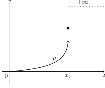
Figure 1: Graph of a solution u .
