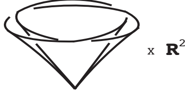
Figure 3: Four-dimensional cuspidal-conical edge
