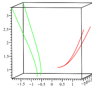
hyperbolic evolute of the hyperbolic 3/2-cusp
