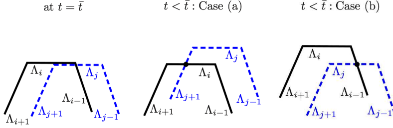
FIG. 9. The case of facet-facet intersection with \Lambda_i(\bar{t}) \not\subset \Lambda_j(\bar{t}) and \Lambda_i(\bar{t}) \not\supset \Lambda_j(\bar{t}) .
