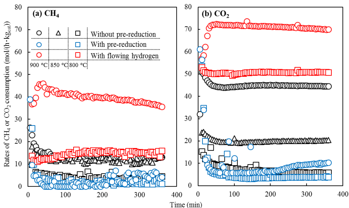
Figure 3-3 Rates of (a): \text{CH}_4 and (b): \text{CO}_2 consumption during the catalytic tests without reduction (black, \text{Ar}:\text{CH}_4:\text{CO}_2 = 8:1:1 ), the catalytic test with pre-reduction (blue, \text{Ar}:\text{CH}_4:\text{CO}_2 = 8:1:1 ), and the catalytic test with flowing hydrogen (red, \text{Ar}:\text{H}_2:\text{CH}_4:\text{CO}_2 = 7:1:1:1 ). The temperature was 800–900 °C and the gas flow rate was 30 L/(h·g cat ). The difference in the catalytic performances is likely related to the state of the limonite ore catalyst. Figure 3-5 (a) shows XRD patterns of the limonite ore catalysts before and after the catalytic tests and Figure 3-5 (b) shows the detailed XRD patterns of the catalysts after the catalytic tests with flowing hydrogen at 2\theta = 44\text{--}45^\circ .
