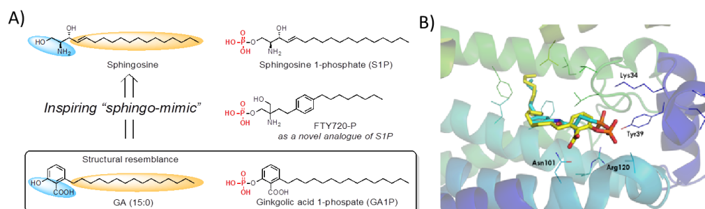
A) Our new concept GA inspires “sphingo-mimic”: Structural resemblance between GA and sphingosine. B) In silico docking model of GA1P (yellow) with bound ligand ML5 (cyan) to S1P 1 .
