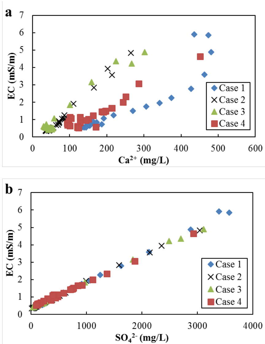
Figure 6 Electrical conductivity vs concentrations of (a) \text{Ca}^{2+} and (b) \text{SO}_4^{2-}
