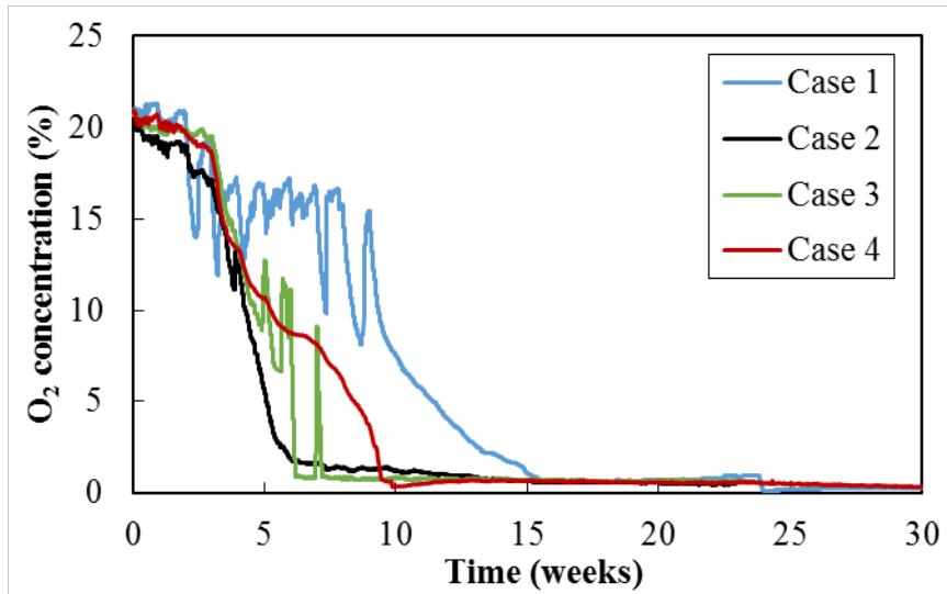
Figure 4 Changes of oxygen concentration
