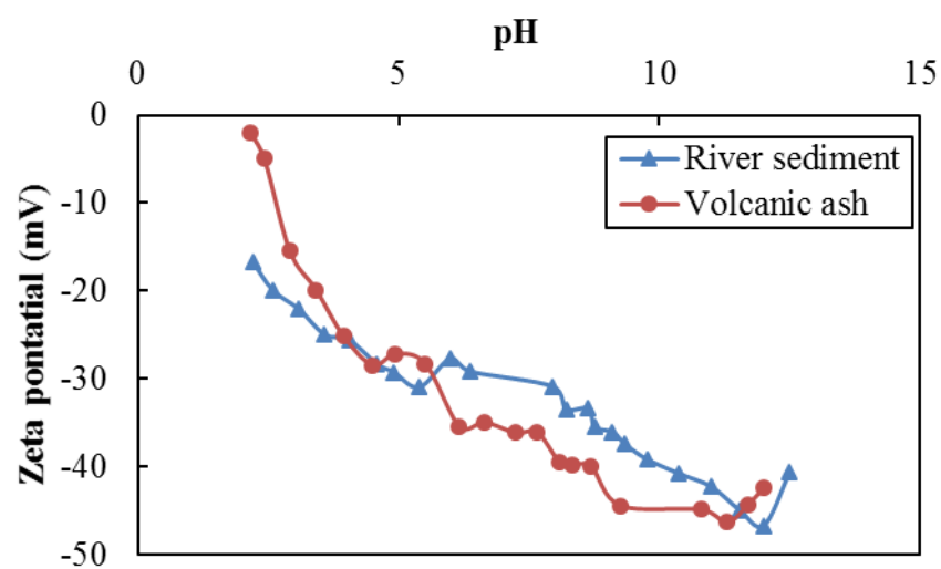
Figure 2 Zeta potential vs pH of river sediment and volcanic ash
