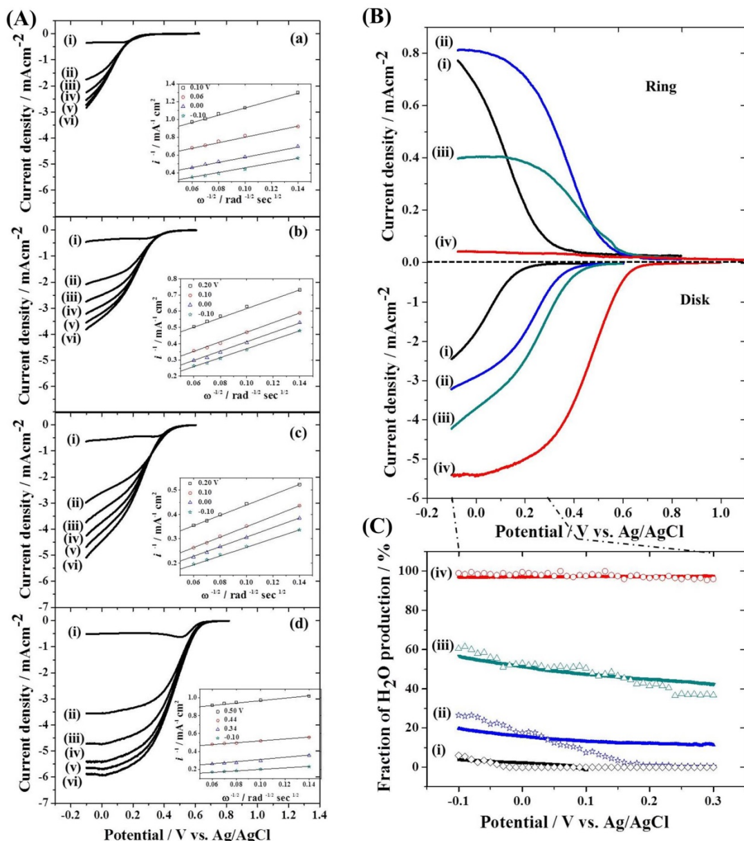
Figure 2. (A) LSVs of (a) bare Au, (b) BNNS/Au, (c) Au-BNNS/Au, and (d) Pt electrodes in O 2 saturated 0.5 M H 2 SO 4 solution in RDE configuration with rotation rate of (i) 0, (ii) 500, (iii) 1000, (iv) 1500, (v) 2000, and (vi) 2500 rpm. Sweep rate: 10 mV/s. Insets: K-L plots of each electrode at various potentials. (B) Disk current at (i) bare Au, (ii) BNNS/Au, (iii) Au-BNNS/Au, and (iv) bare Pt electrodes (bottom panel) and corresponding ring current at a Pt ring electrode held at 900 mV (top panel) in RRDE configuration with the rotation rate of 1500 rpm as a function of disk potential measured in O 2 saturated 0.5 M H 2 SO 4 solution with the sweep rate of 10mV/sec. (C) Fraction of H 2 O generation as a function of potential at (i) bare Au, (ii) BNNS/Au, (iii) Au-BNNS/Au, and (iv) Pt electrodes determined from K-L plots (Figure 2(A)) (symbols) and RRDE (Figure 2(B)) measurements (solid lines).
