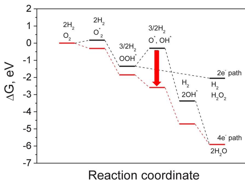
Figure: 3 Free energy diagrams for ORR at BN monolayer/Au(111) (black line) and Au 8 -BN monolayer/Au(111) (red line) electrodes.
