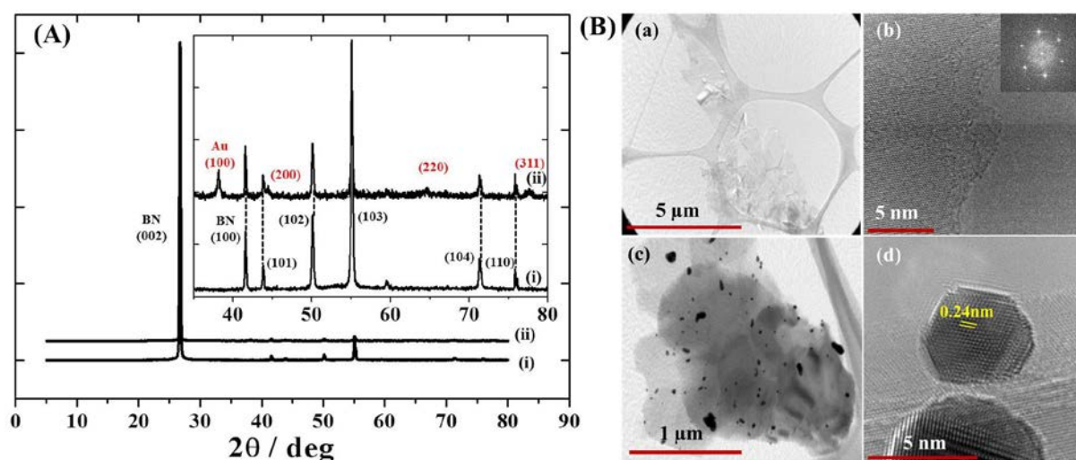
Figure1. (A) XRD patterns of (i) BNNS and (ii) Au-BNNS. Inset: Enlarged patterns. Diffraction peaks are marked by black and red for BN and Au peaks, respectively. (B) TEM images of BNNS ((a), (b)) and Au-BNNS ((c), (d)). Inset of (b) is the FFT of the central part of the image.
