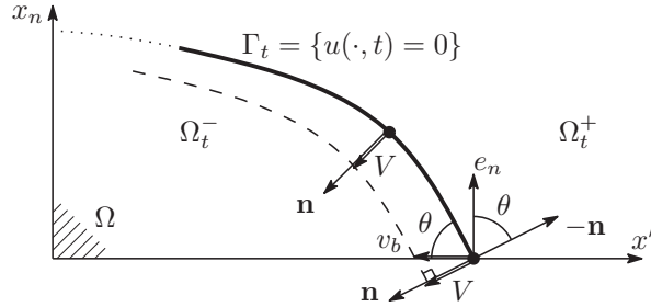
Figure 1: Interface problem
