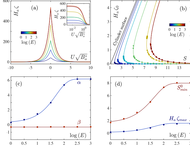
Figure 2: (a) Surface profiles for different values of the minimum separation distance S_{min}^0 , given by the corresponding dimensionless thickness E (in colors). The inset shows the U > 0 side in log – log scale. (b) Apex position \zeta_0 as a function of the separation distance S , for different E (in colors). Lines correspond to eq. (30). (c) Parameters \alpha and \beta as functions of E . The two lines are \alpha given by a saturating exponential (see text) and \beta = -0.3 . (d) Maximum apex position \zeta_{max} and S_{min}^0 as functions of E . Lines correspond to eqs. (30–31).
