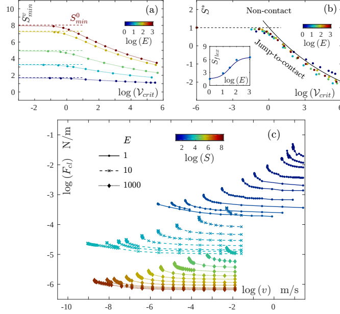
Figure 5: (a) Minimum separation distance S_{min}^v as a function of the critical speed V_{crit} , for different values of the dimensionless thickness E (in colors). Dashed lines represent the values of S_{min}^0 in the static limit V = 0 , for each E . (b) Phase diagram which interface is given by the reduced separation distance S^* , defined in eq. (32), and V_{crit} . The continuous line corresponds to the JTC threshold, given by eq. (34), and the dashed line represents the static value S_{min}^0 . The inset shows the separation distance of the inflection point S_{flex} , for each curve in (a), as a function of E . The continuous line corresponds to eq. (33). (c) Probe-liquid force F_{cl} per unit length as a function of the probe speed v , for different values of S and E .
