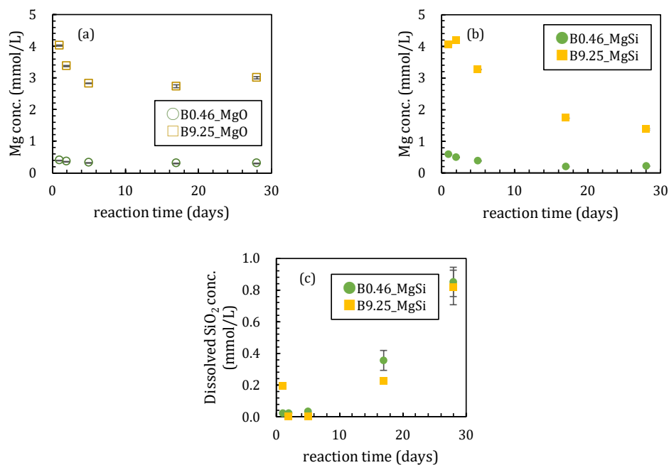
Figure 3. Changes of concentration of dissolved species; (a) Mg without amorphous silica, (b) Mg and (c) SiO 2 with amorphous silica. Data with error bars indicate the standard error of three samples.
