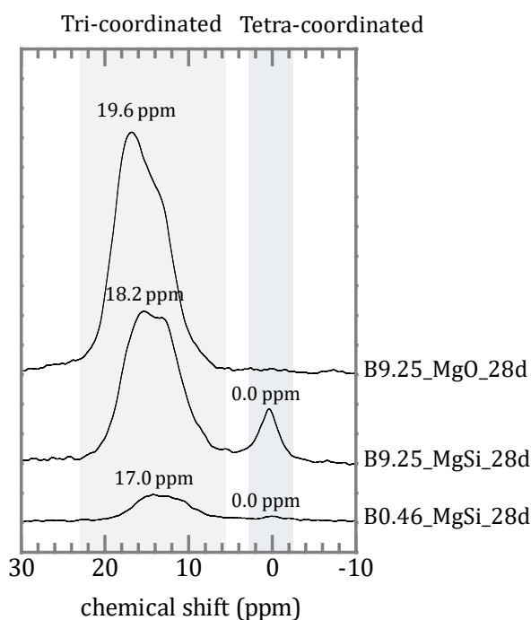
Figure 7. ^{11}\text{B} magic-angle spinning nuclear magnetic resonance (MAS-NMR) spectra of 28-day aged samples with [\text{B}]_{\text{ini}} = 0.46 mmol/L and silica (bottom spectrum), and with [\text{B}]_{\text{ini}} = 9.25 mmol/L with (mid) and without silica (top) all aged for 28 days.
