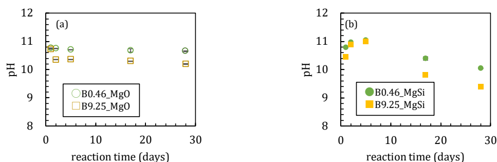
Figure 2. Changes in pH during sorption for (a) without amorphous silica and (b) with amorphous silica. Data with error bars indicate the standard error of three samples.
