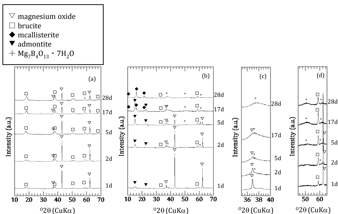
Figure 4. X-ray diffractometry (XRD) spectra of samples without amorphous silica; (a) [B]_{ini} = 0.46 mmol/L and (b) [B]_{ini} = 9.25 mmol/L with magnified (b) spectra for (c) 35–40° and (d) 45–65° in 2\theta .
