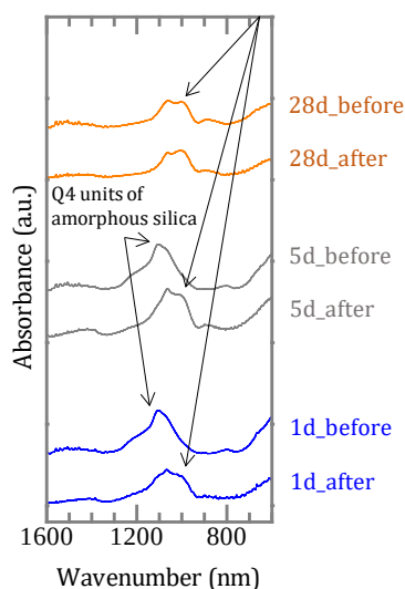
Figure 10. FT-IR spectra of precipitates before and after boron sorption.
