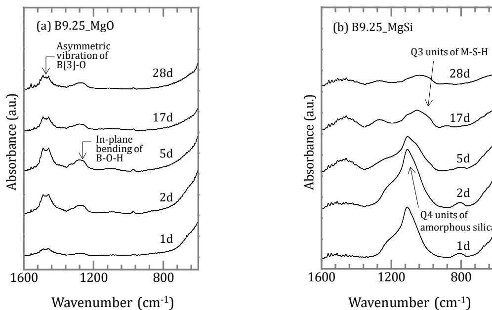
Figure 6. Fourier transform infrared spectrometer (FT-IR) spectra of samples (a) without amorphous silica and (b) with amorphous silica.
