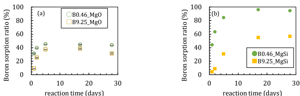
Figure 1. Changes of boron sorption ratios with time for the sorption of 0.46 and 9.25 mmol/L boron on MgO (a) without amorphous silica and (b) with amorphous silica. Data with error bars indicate the standard error of three samples.
