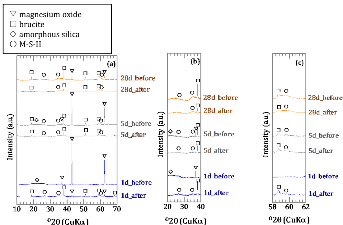
Figure 9. XRD spectra of precipitates (a) before and after sorption with magnified spectra shown in (a) for (b) 20\text{--}40^\circ and (c) 58\text{--}62^\circ in 2\theta .
