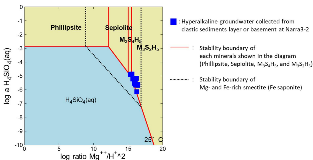
Figure 8. Phase diagram for the Mg-Si-Fe-Al-Na system. Blue squares represent hyperalkaline groundwater collected from the clastic sediment layer or basement at Narra3-2. Dotted lines show stability boundaries of Mg- and Fe-rich smectite (Fe saponite). \text{M}_3\text{S}_4\text{H}_5 : M-S-H ( 3\text{MgO} \cdot 4\text{SiO}_2 \cdot 5\text{H}_2\text{O} ); \text{M}_3\text{S}_2\text{H}_5 : M-S-H ( 3\text{MgO} \cdot 2\text{SiO}_2 \cdot 5\text{H}_2\text{O} ).
