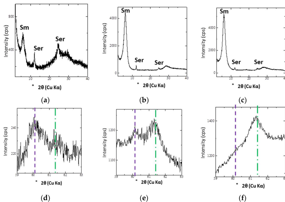
Figure 5. XRD traces of the <2\ \mu\text{m} fraction of DH4 at different depths: (a) Oriented XRD traces at 3 m; (b) Oriented XRD traces at 6 m; (c) Oriented XRD traces at 10 m; (d) XRD traces of the 060 reflection at 3 m; (e) XRD traces of the 060 reflection at 6 m; (f) XRD traces of the 060 reflection at 10 m. Sm: smectite; Ser: serpentine.
